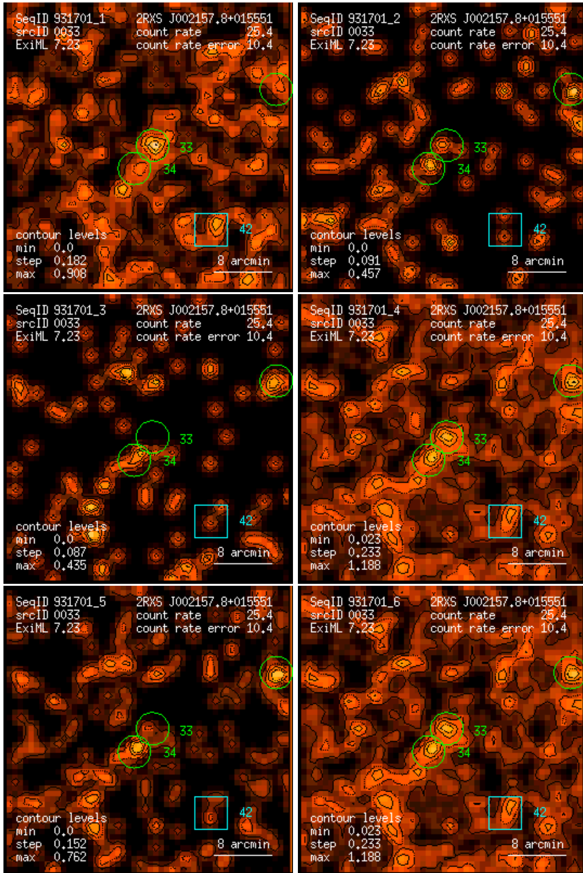
Figure 33: RASS 931701: detection 0033: band rate images, Gaussian filter: (1) PSPC channels 11 – 41, (2) 52 – 90, (3) 91 – 201, (4) 11 – 235, (5) 52 – 201, (6) 11 – 201. Broad band rates in counts/ks. Band rate contour levels in counts/ks/arcmin 2 .
