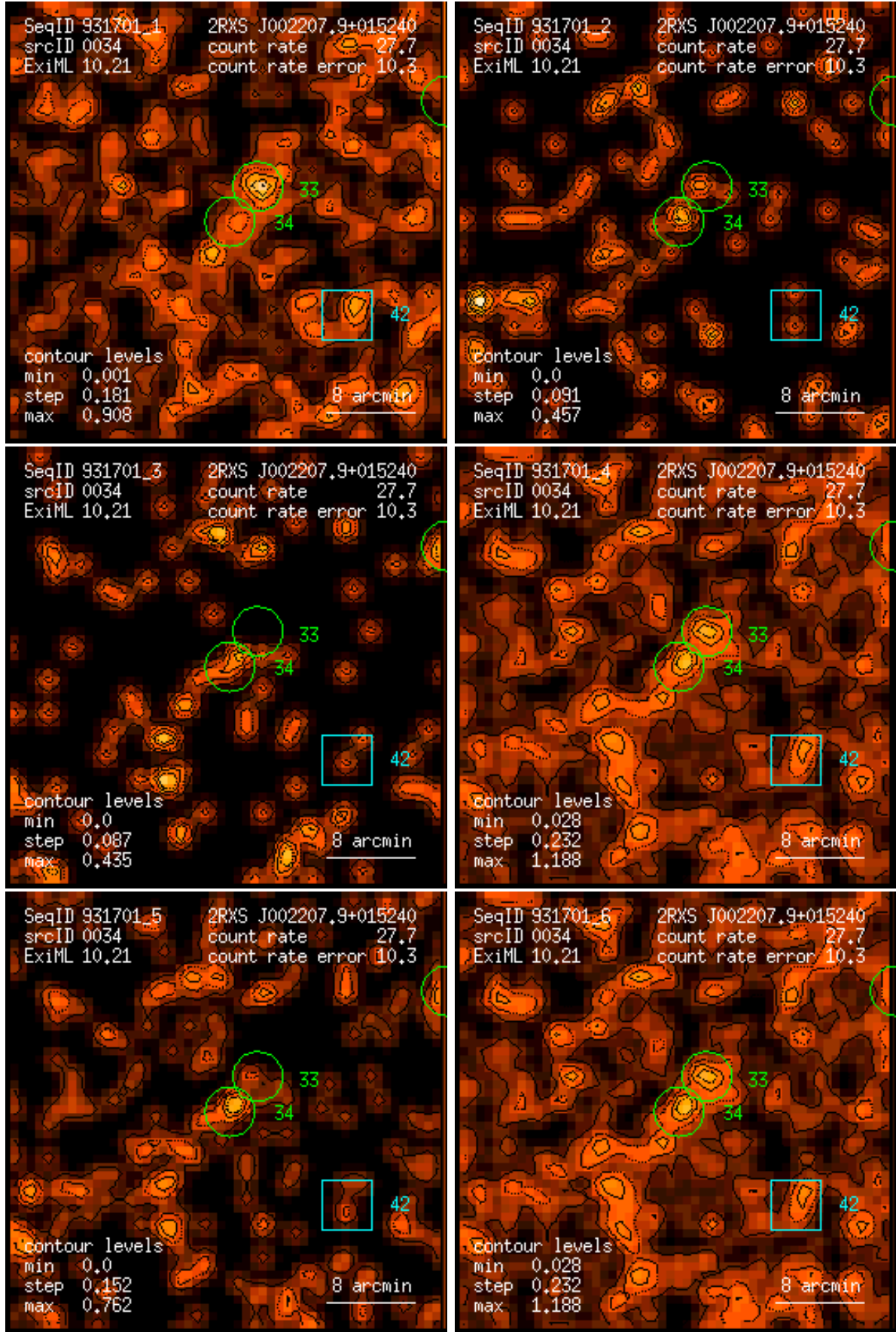
Figure 34: RASS 931701: detection 0034: band rate images, Gaussian filter: (1) PSPC channels 11 – 41, (2) 52 – 90, (3) 91 – 201, (4) 11 – 235, (5) 52 – 201, (6) 11 – 201. Broad band rates in counts/ks. Band rate contour levels in counts/ks/arcmin 2 .
