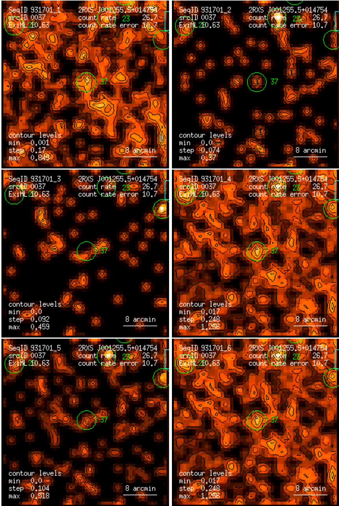
Figure 37: RASS 931701: detection 0037: band rate images, Gaussian filter: (1) PSPC channels 11 – 41, (2) 52 – 90, (3) 91 – 201, (4) 11 – 235, (5) 52 – 201, (6) 11 – 201. Broad band rates in counts/ks. Band rate contour levels in counts/ks/arcmin 2 .
