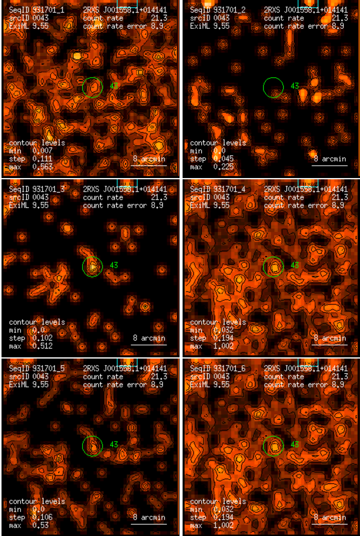
Figure 43: RASS 931701: detection 0043: band rate images, Gaussian filter: (1) PSPC channels 11 – 41, (2) 52 – 90, (3) 91 – 201, (4) 11 – 235, (5) 52 – 201, (6) 11 – 201. Broad band rates in counts/ks. Band rate contour levels in counts/ks/arcmin 2 .
