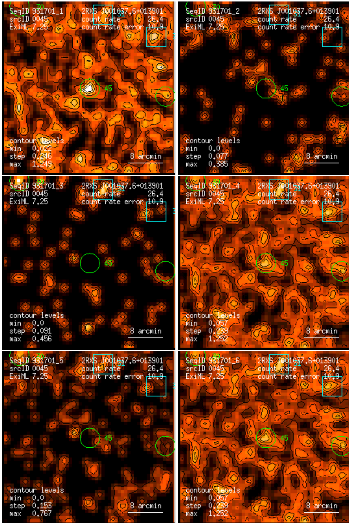
Figure 45: RASS 931701: detection 0045: band rate images, Gaussian filter: (1) PSPC channels 11 – 41, (2) 52 – 90, (3) 91 – 201, (4) 11 – 235, (5) 52 – 201, (6) 11 – 201. Broad band rates in counts/ks. Band rate contour levels in counts/ks/arcmin 2 .
