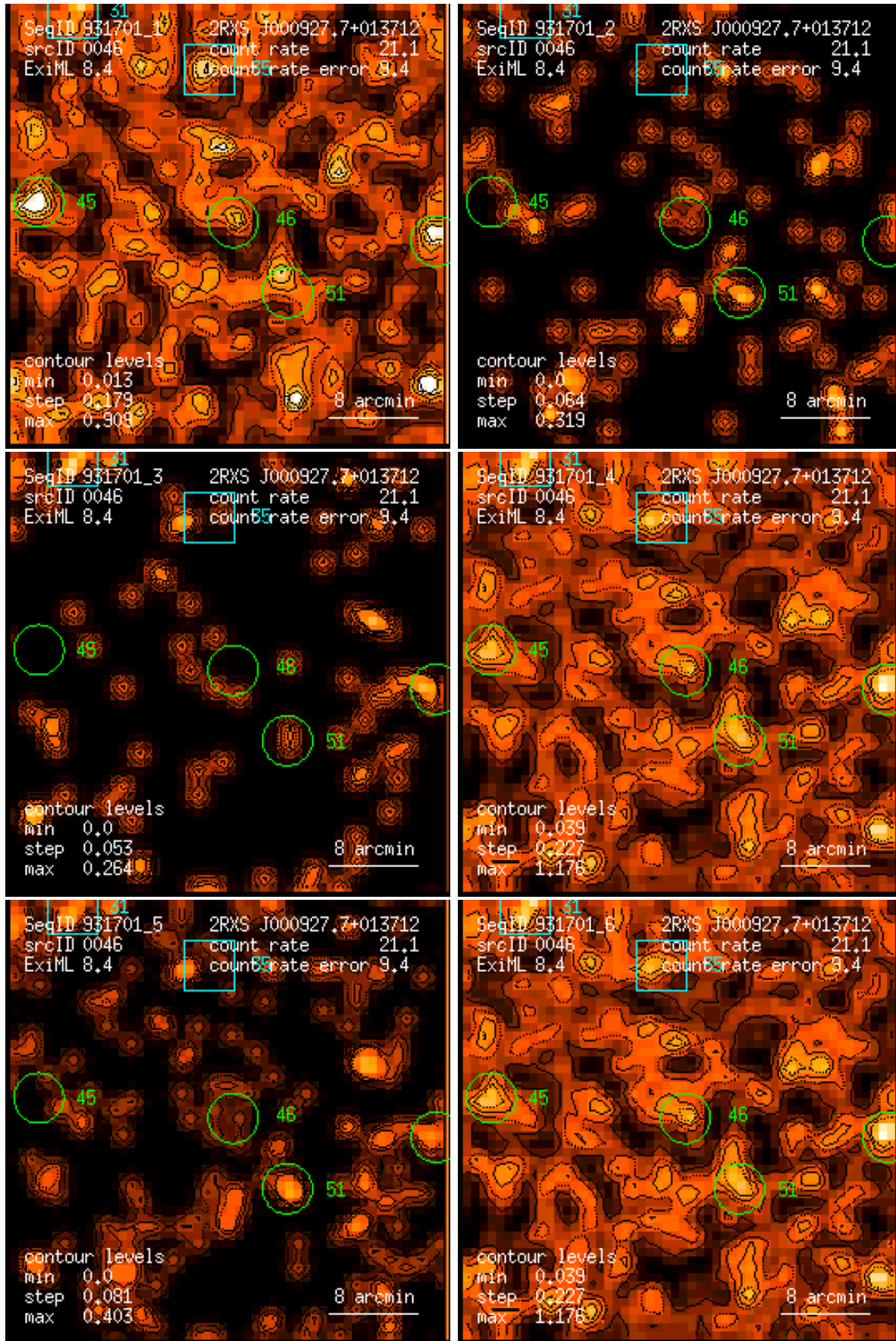
Figure 46: RASS 931701: detection 0046: band rate images, Gaussian filter: (1) PSPC channels 11 – 41, (2) 52 – 90, (3) 91 – 201, (4) 11 – 235, (5) 52 – 201, (6) 11 – 201. Broad band rates in counts/ks. Band rate contour levels in counts/ks/arcmin 2 .
