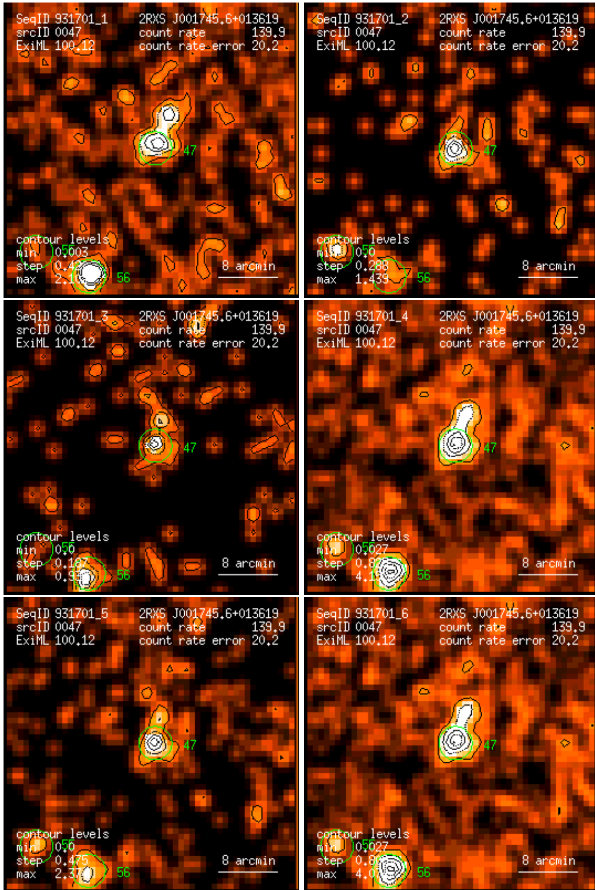
Figure 47: RASS 931701: detection 0047: band rate images, Gaussian filter: (1) PSPC channels 11 – 41, (2) 52 – 90, (3) 91 – 201, (4) 11 – 235, (5) 52 – 201, (6) 11 – 201. Broad band rates in counts/ks. Band rate contour levels in counts/ks/arcmin 2 .
