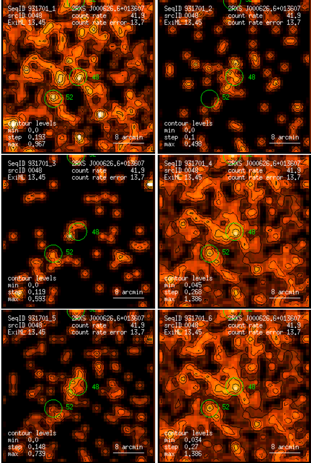
Figure 48: RASS 931701: detection 0048: band rate images, Gaussian filter: (1) PSPC channels 11 – 41, (2) 52 – 90, (3) 91 – 201, (4) 11 – 235, (5) 52 – 201, (6) 11 – 201. Broad band rates in counts/ks. Band rate contour levels in counts/ks/arcmin 2 .
