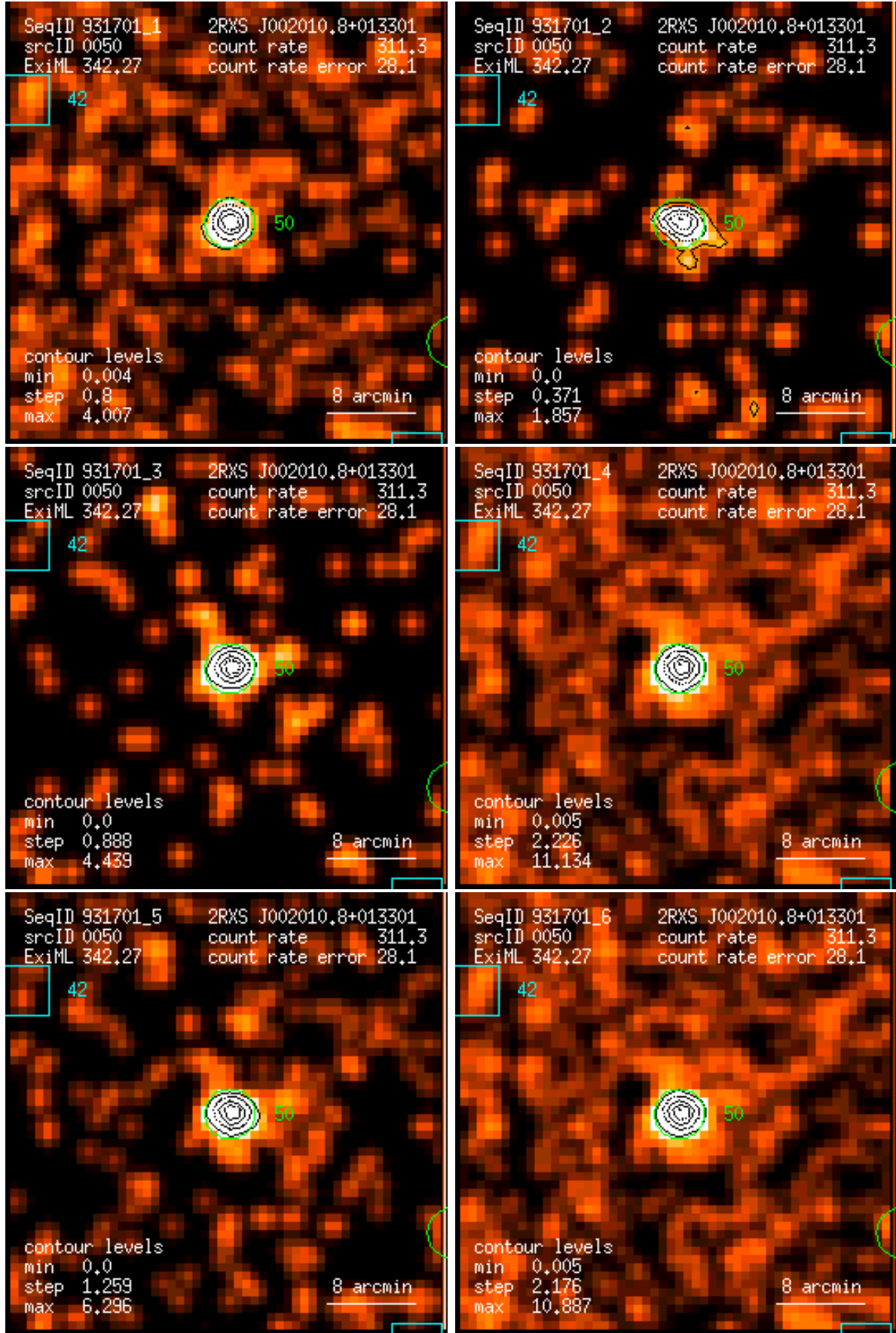
Figure 50: RASS 931701: detection 0050: band rate images, Gaussian filter: (1) PSPC channels 11 – 41, (2) 52 – 90, (3) 91 – 201, (4) 11 – 235, (5) 52 – 201, (6) 11 – 201. Broad band rates in counts/ks. Band rate contour levels in counts/ks/arcmin 2 .
