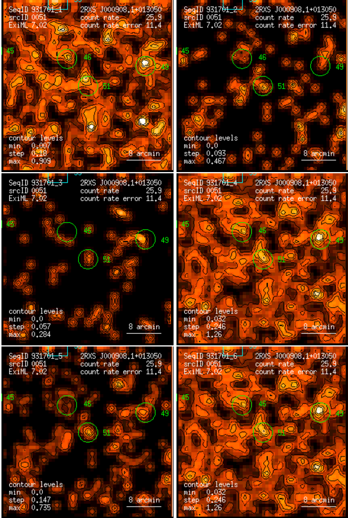
Figure 51: RASS 931701: detection 0051: band rate images, Gaussian filter: (1) PSPC channels 11 – 41, (2) 52 – 90, (3) 91 – 201, (4) 11 – 235, (5) 52 – 201, (6) 11 – 201. Broad band rates in counts/ks. Band rate contour levels in counts/ks/arcmin 2 .
