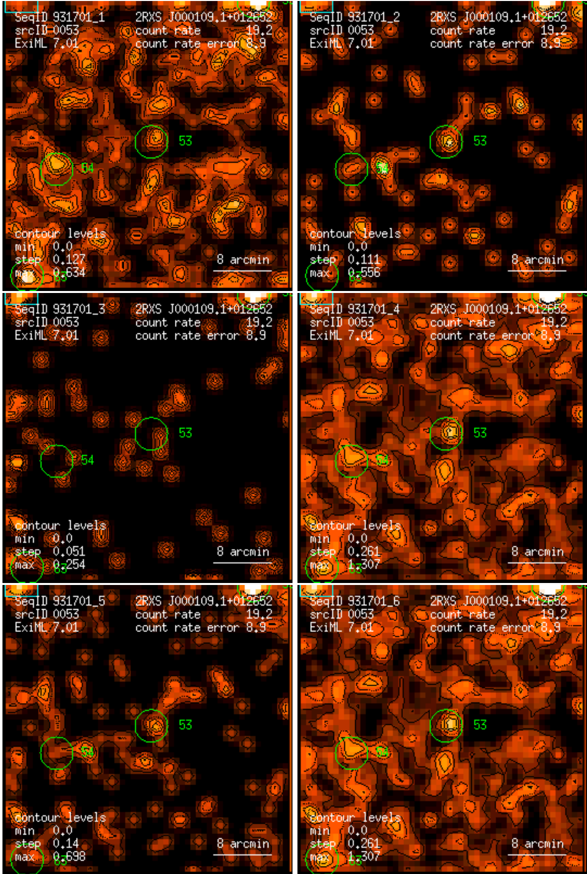
Figure 53: RASS 931701: detection 0053: band rate images, Gaussian filter: (1) PSPC channels 11 – 41, (2) 52 – 90, (3) 91 – 201, (4) 11 – 235, (5) 52 – 201, (6) 11 – 201. Broad band rates in counts/ks. Band rate contour levels in counts/ks/arcmin 2 .
