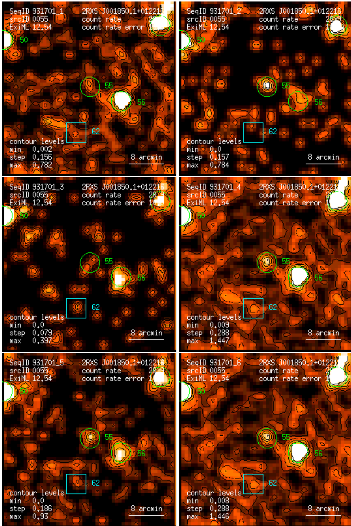
Figure 55: RASS 931701: detection 0055: band rate images, Gaussian filter: (1) PSPC channels 11 – 41, (2) 52 – 90, (3) 91 – 201, (4) 11 – 235, (5) 52 – 201, (6) 11 – 201. Broad band rates in counts/ks. Band rate contour levels in counts/ks/arcmin 2 .
