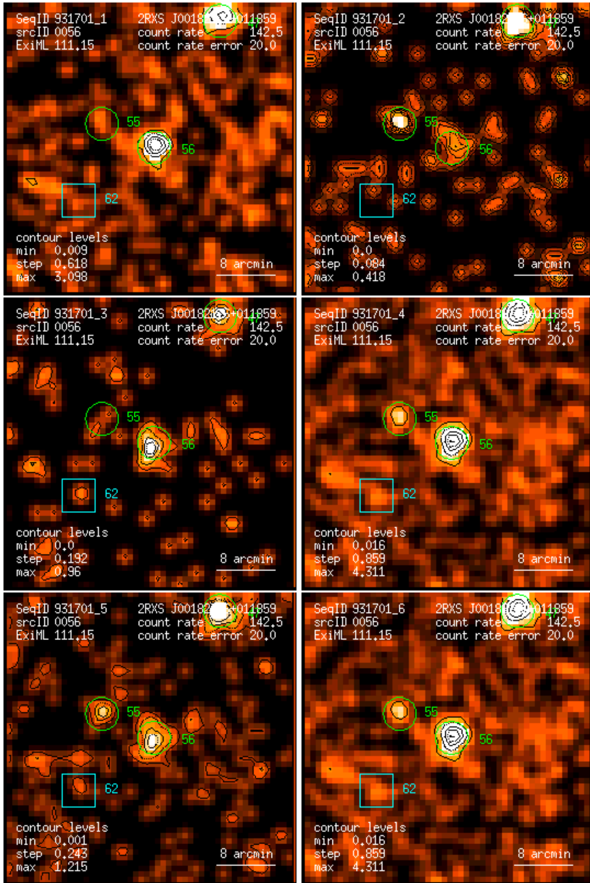
Figure 56: RASS 931701: detection 0056: band rate images, Gaussian filter: (1) PSPC channels 11 – 41, (2) 52 – 90, (3) 91 – 201, (4) 11 – 235, (5) 52 – 201, (6) 11 – 201. Broad band rates in counts/ks. Band rate contour levels in counts/ks/arcmin 2 .
