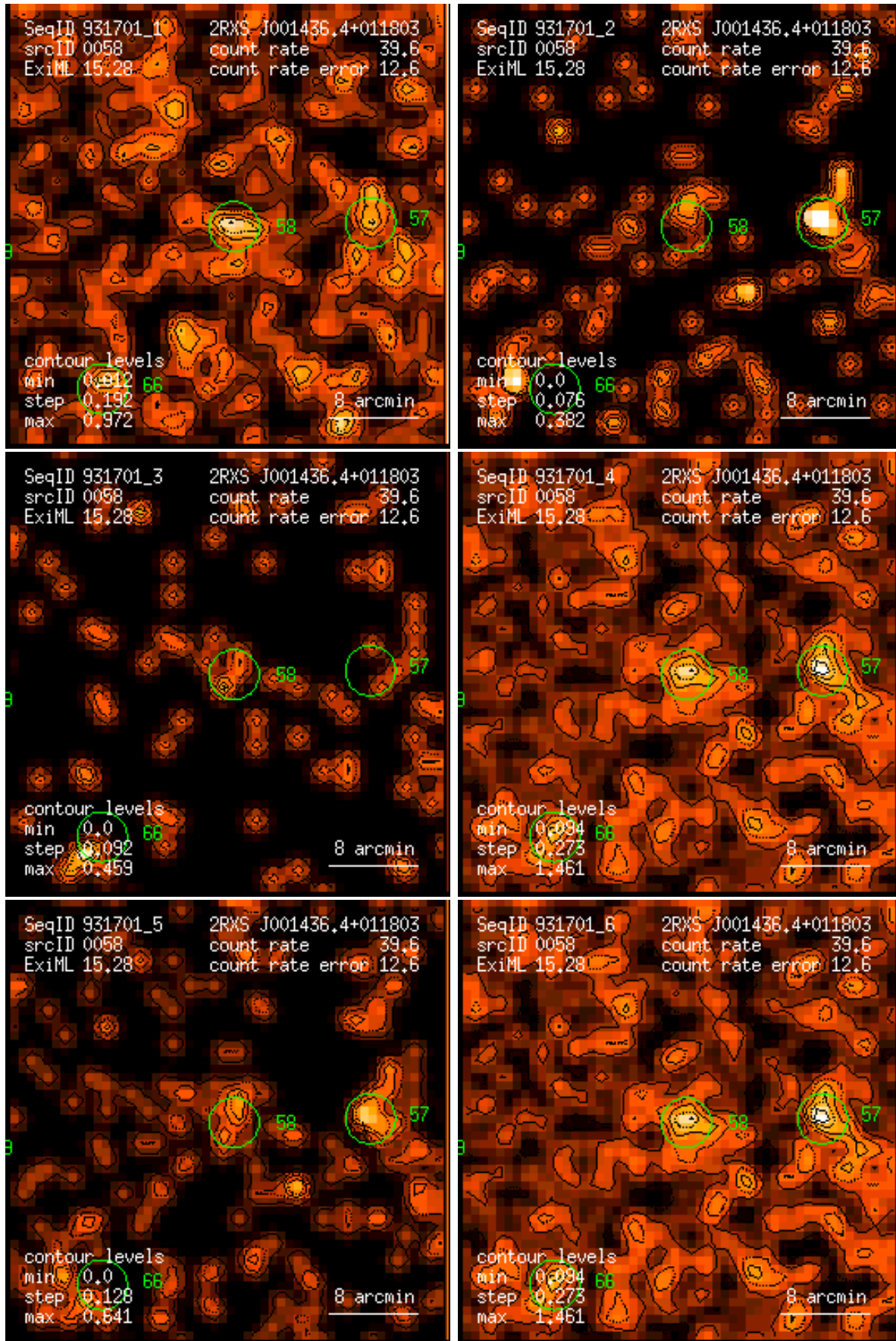
Figure 58: RASS 931701: detection 0058: band rate images, Gaussian filter: (1) PSPC channels 11 – 41, (2) 52 – 90, (3) 91 – 201, (4) 11 – 235, (5) 52 – 201, (6) 11 – 201. Broad band rates in counts/ks. Band rate contour levels in counts/ks/arcmin 2 .
