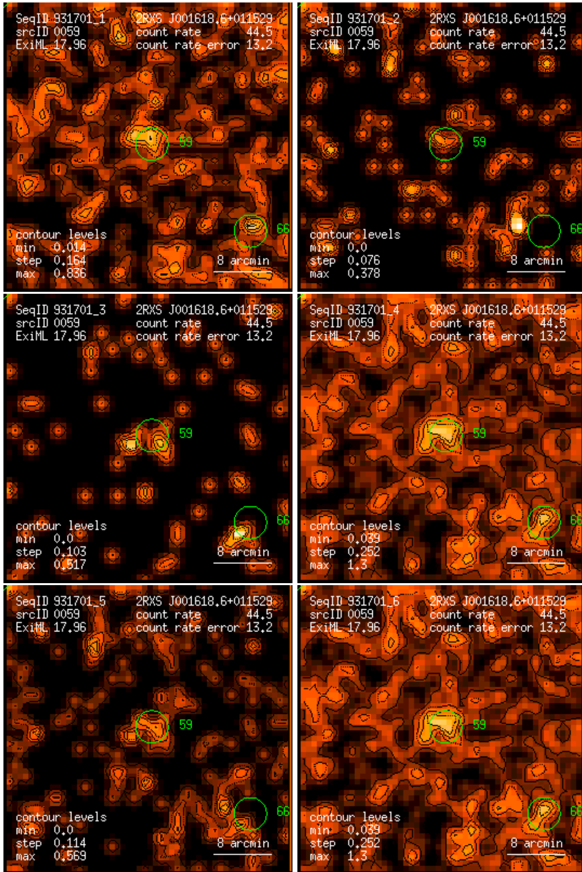
Figure 59: RASS 931701: detection 0059: band rate images, Gaussian filter: (1) PSPC channels 11 – 41, (2) 52 – 90, (3) 91 – 201, (4) 11 – 235, (5) 52 – 201, (6) 11 – 201. Broad band rates in counts/ks. Band rate contour levels in counts/ks/arcmin 2 .
