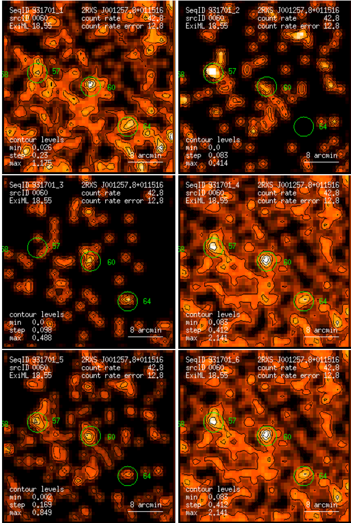
Figure 60: RASS 931701: detection 0060: band rate images, Gaussian filter: (1) PSPC channels 11 – 41, (2) 52 – 90, (3) 91 – 201, (4) 11 – 235, (5) 52 – 201, (6) 11 – 201. Broad band rates in counts/ks. Band rate contour levels in counts/ks/arcmin 2 .
