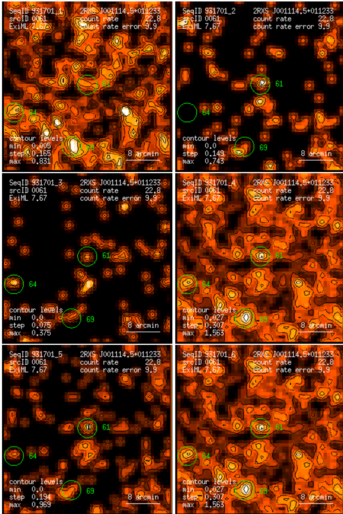
Figure 61: RASS 931701: detection 0061: band rate images, Gaussian filter: (1) PSPC channels 11 – 41, (2) 52 – 90, (3) 91 – 201, (4) 11 – 235, (5) 52 – 201, (6) 11 – 201. Broad band rates in counts/ks. Band rate contour levels in counts/ks/arcmin 2 .
