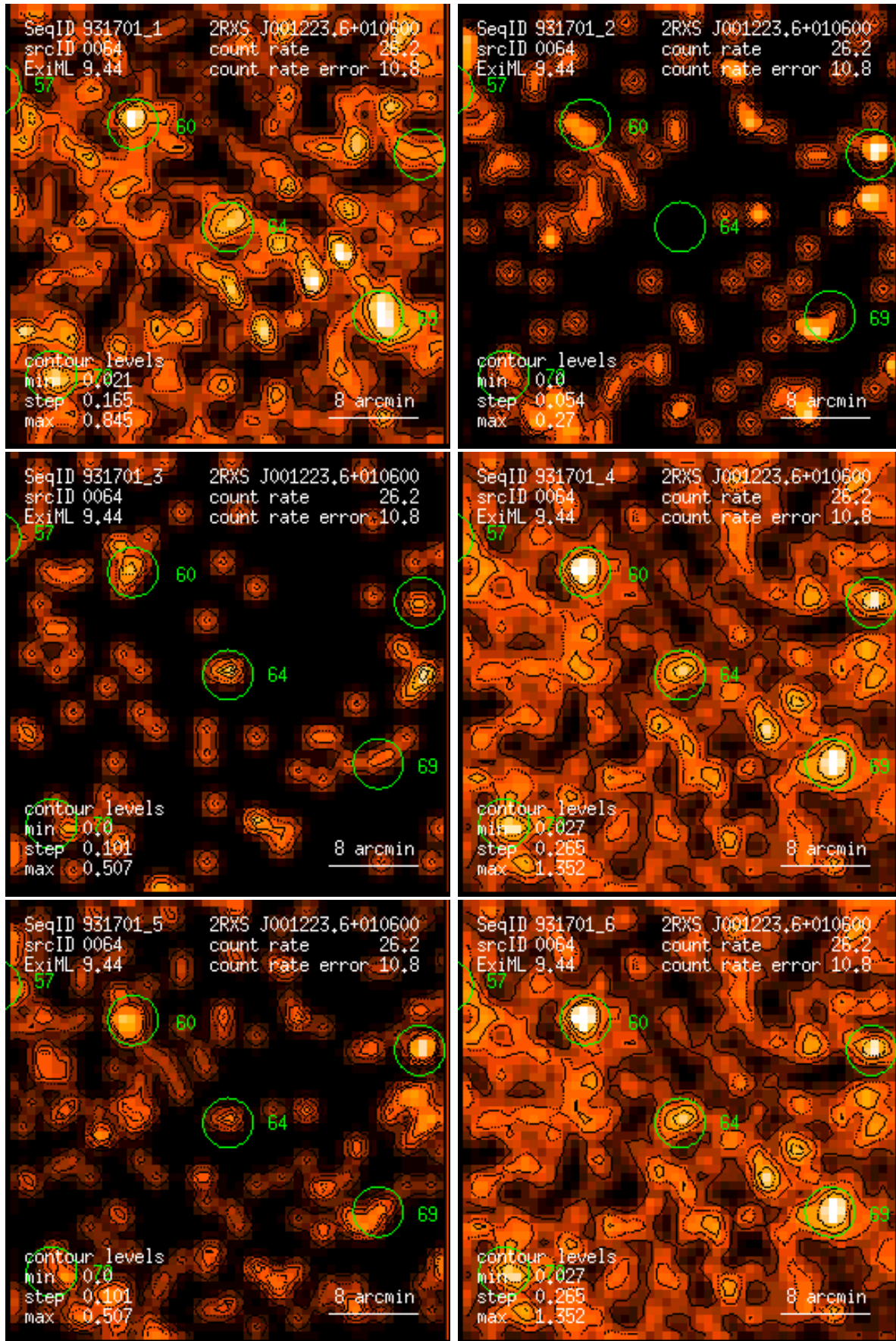
Figure 64: RASS 931701: detection 0064: band rate images, Gaussian filter: (1) PSPC channels 11 – 41, (2) 52 – 90, (3) 91 – 201, (4) 11 – 235, (5) 52 – 201, (6) 11 – 201. Broad band rates in counts/ks. Band rate contour levels in counts/ks/arcmin 2 .
