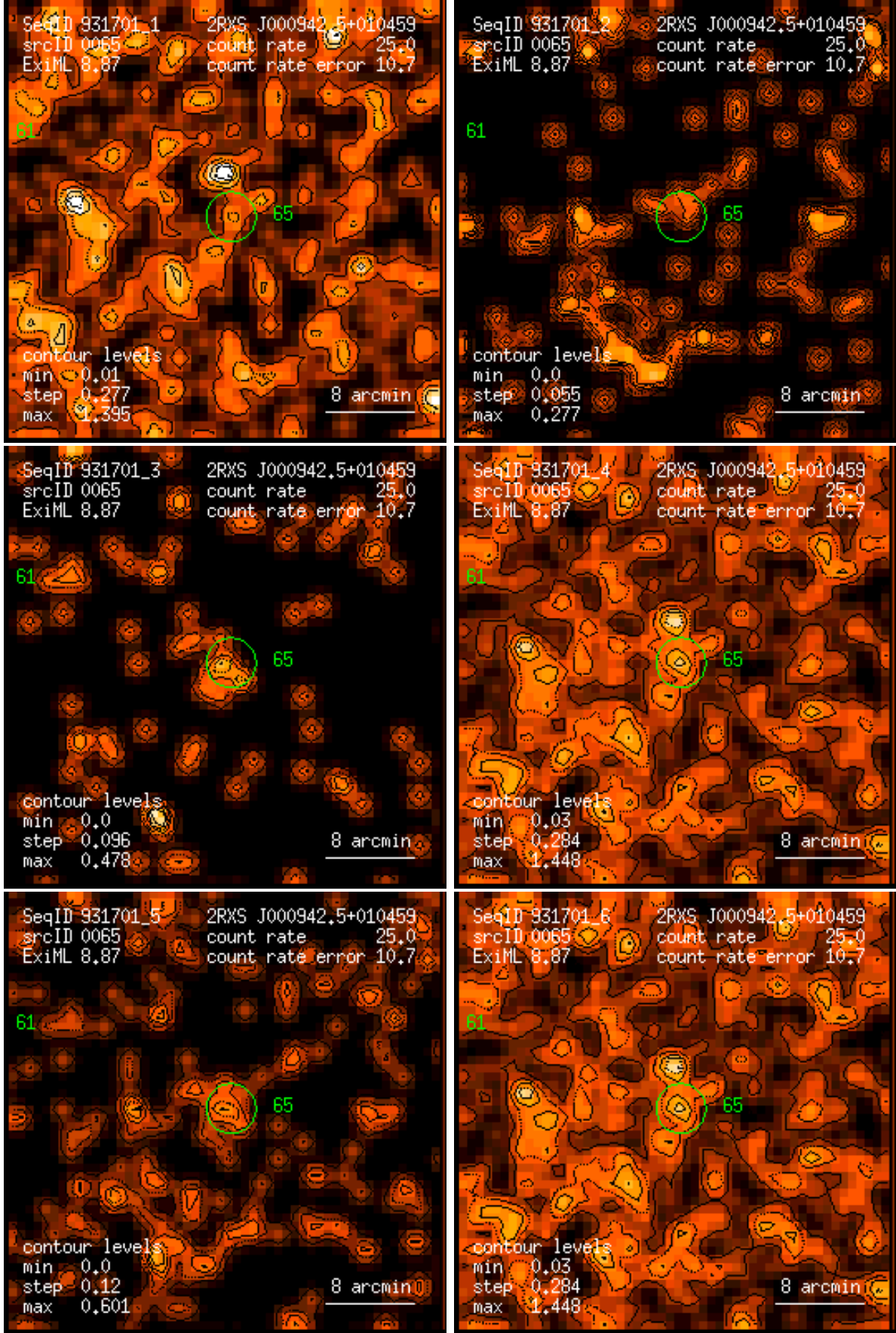
Figure 65: RASS 931701: detection 0065: band rate images, Gaussian filter: (1) PSPC channels 11 – 41, (2) 52 – 90, (3) 91 – 201, (4) 11 – 235, (5) 52 – 201, (6) 11 – 201. Broad band rates in counts/ks. Band rate contour levels in counts/ks/arcmin 2 .
