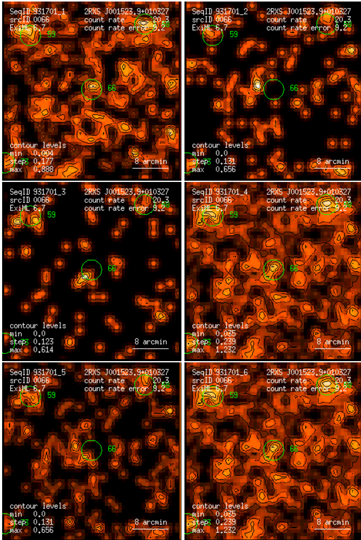
Figure 66: RASS 931701: detection 0066: band rate images, Gaussian filter: (1) PSPC channels 11 – 41, (2) 52 – 90, (3) 91 – 201, (4) 11 – 235, (5) 52 – 201, (6) 11 – 201. Broad band rates in counts/ks. Band rate contour levels in counts/ks/arcmin 2 .
