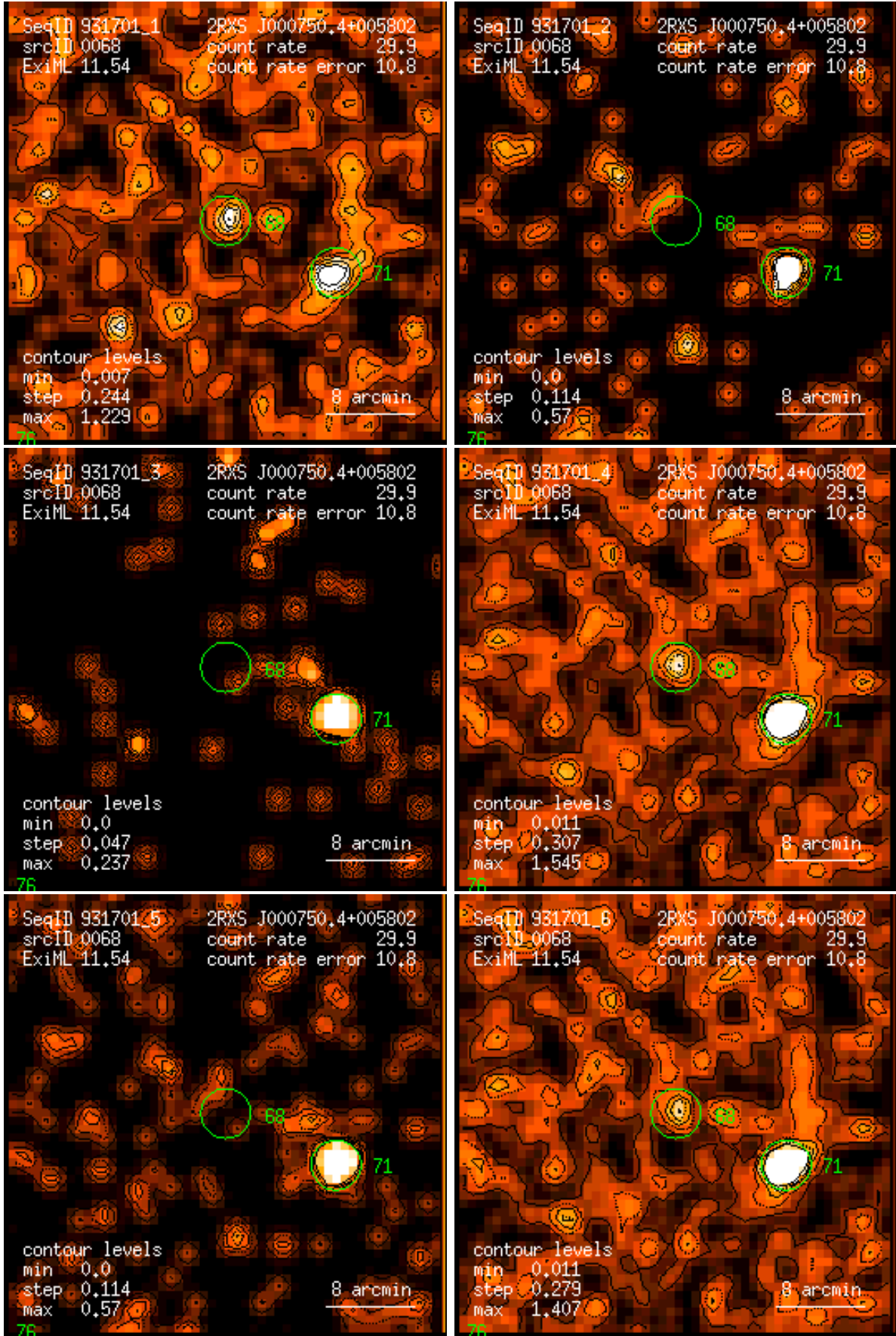
Figure 68: RASS 931701: detection 0068: band rate images, Gaussian filter: (1) PSPC channels 11 – 41, (2) 52 – 90, (3) 91 – 201, (4) 11 – 235, (5) 52 – 201, (6) 11 – 201. Broad band rates in counts/ks. Band rate contour levels in counts/ks/arcmin 2 .
