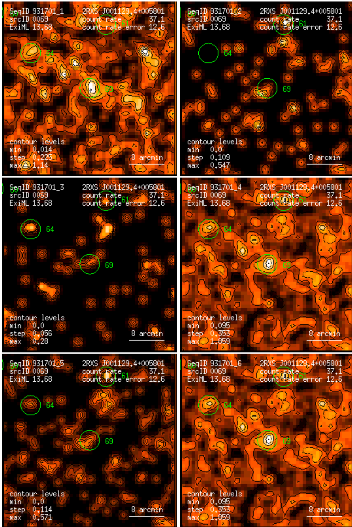
Figure 69: RASS 931701: detection 0069: band rate images, Gaussian filter: (1) PSPC channels 11 – 41, (2) 52 – 90, (3) 91 – 201, (4) 11 – 235, (5) 52 – 201, (6) 11 – 201. Broad band rates in counts/ks. Band rate contour levels in counts/ks/arcmin 2 .
