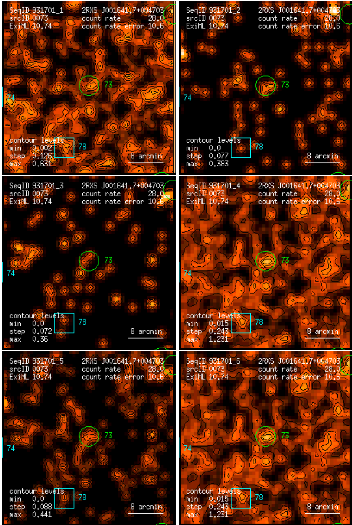
Figure 73: RASS 931701: detection 0073: band rate images, Gaussian filter: (1) PSPC channels 11 – 41, (2) 52 – 90, (3) 91 – 201, (4) 11 – 235, (5) 52 – 201, (6) 11 – 201. Broad band rates in counts/ks. Band rate contour levels in counts/ks/arcmin 2 .
