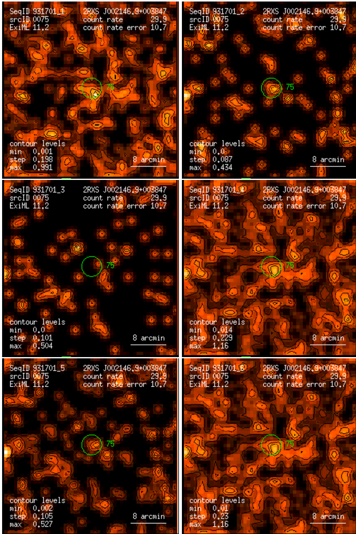
Figure 75: RASS 931701: detection 0075: band rate images, Gaussian filter: (1) PSPC channels 11 – 41, (2) 52 – 90, (3) 91 – 201, (4) 11 – 235, (5) 52 – 201, (6) 11 – 201. Broad band rates in counts/ks. Band rate contour levels in counts/ks/arcmin 2 .
