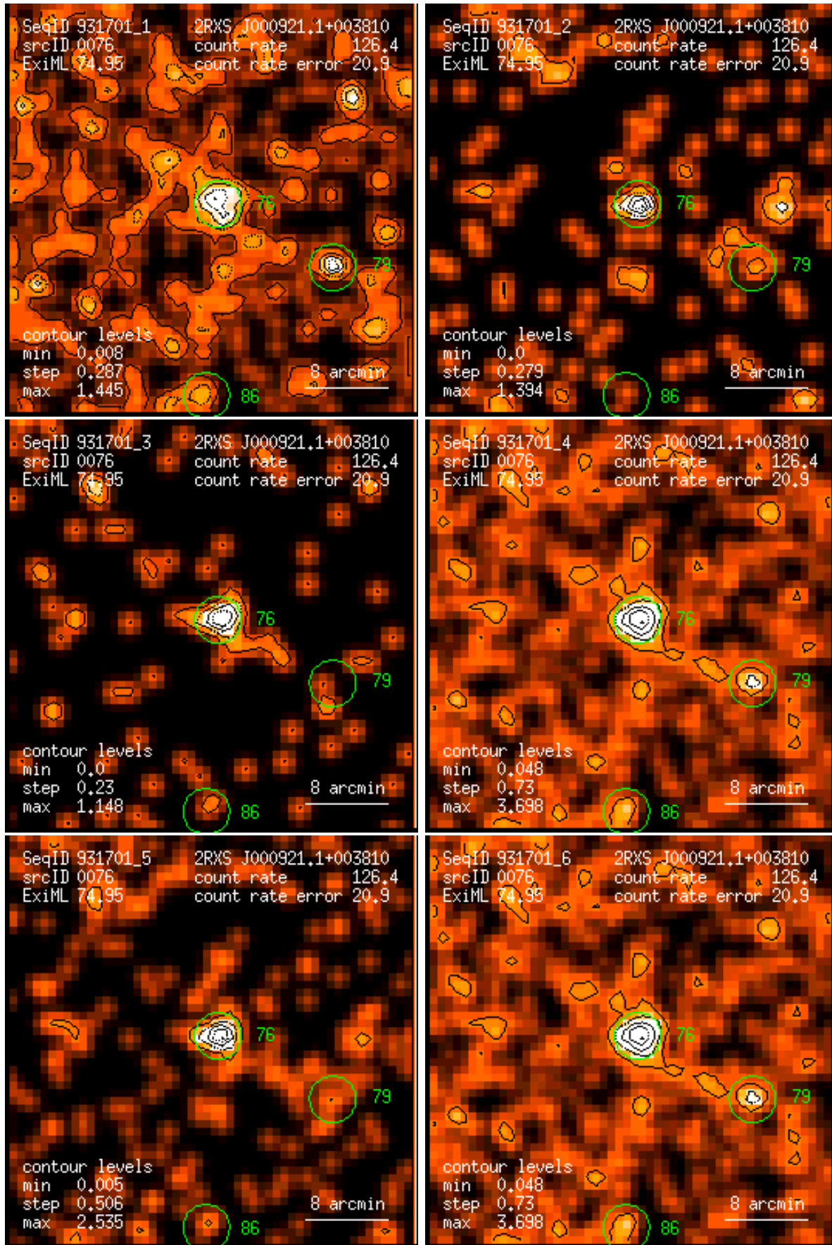
Figure 76: RASS 931701: detection 0076: band rate images, Gaussian filter: (1) PSPC channels 11 – 41, (2) 52 – 90, (3) 91 – 201, (4) 11 – 235, (5) 52 – 201, (6) 11 – 201. Broad band rates in counts/ks. Band rate contour levels in counts/ks/arcmin 2 .
