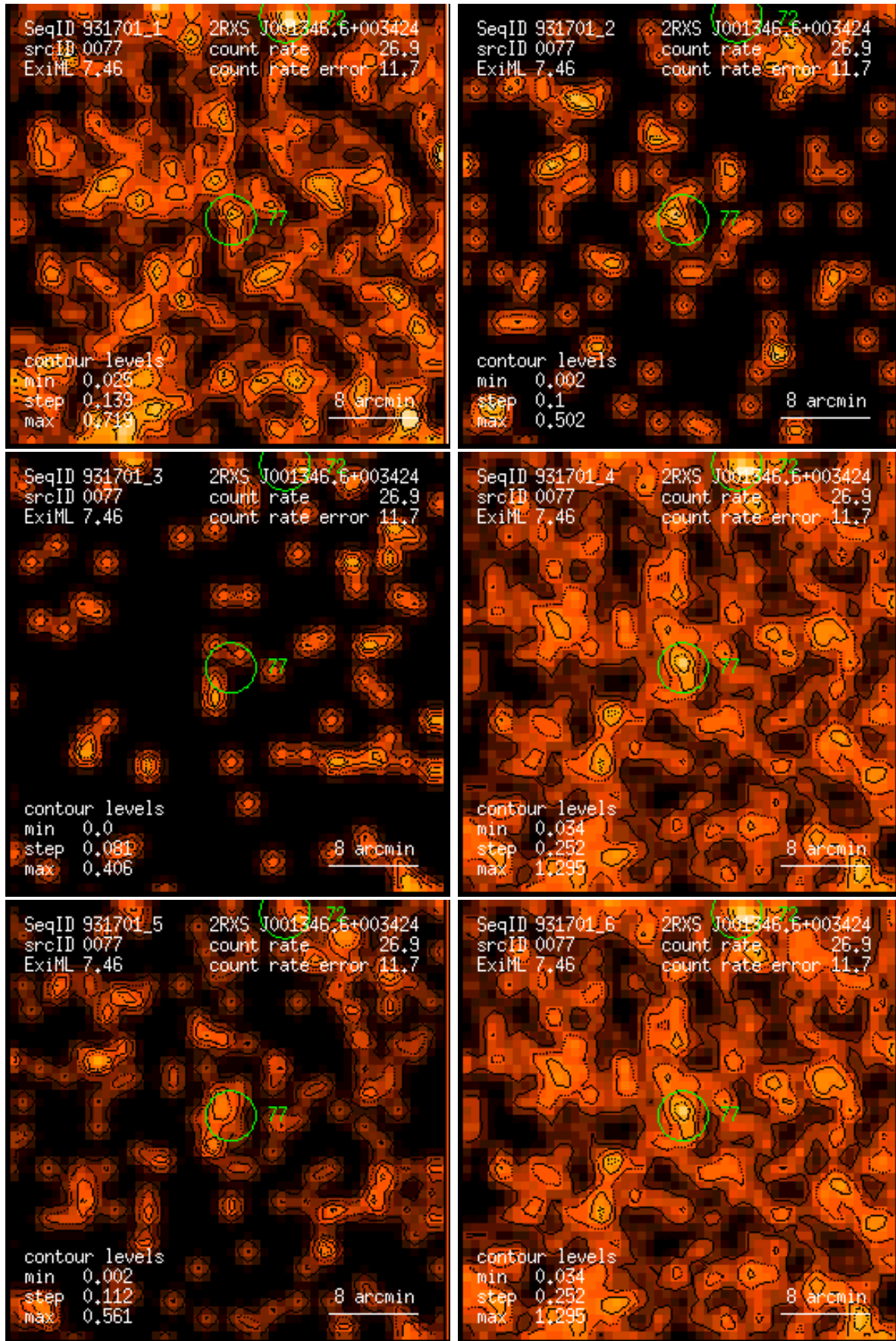
Figure 77: RASS 931701: detection 0077: band rate images, Gaussian filter: (1) PSPC channels 11 – 41, (2) 52 – 90, (3) 91 – 201, (4) 11 – 235, (5) 52 – 201, (6) 11 – 201. Broad band rates in counts/ks. Band rate contour levels in counts/ks/arcmin 2 .
