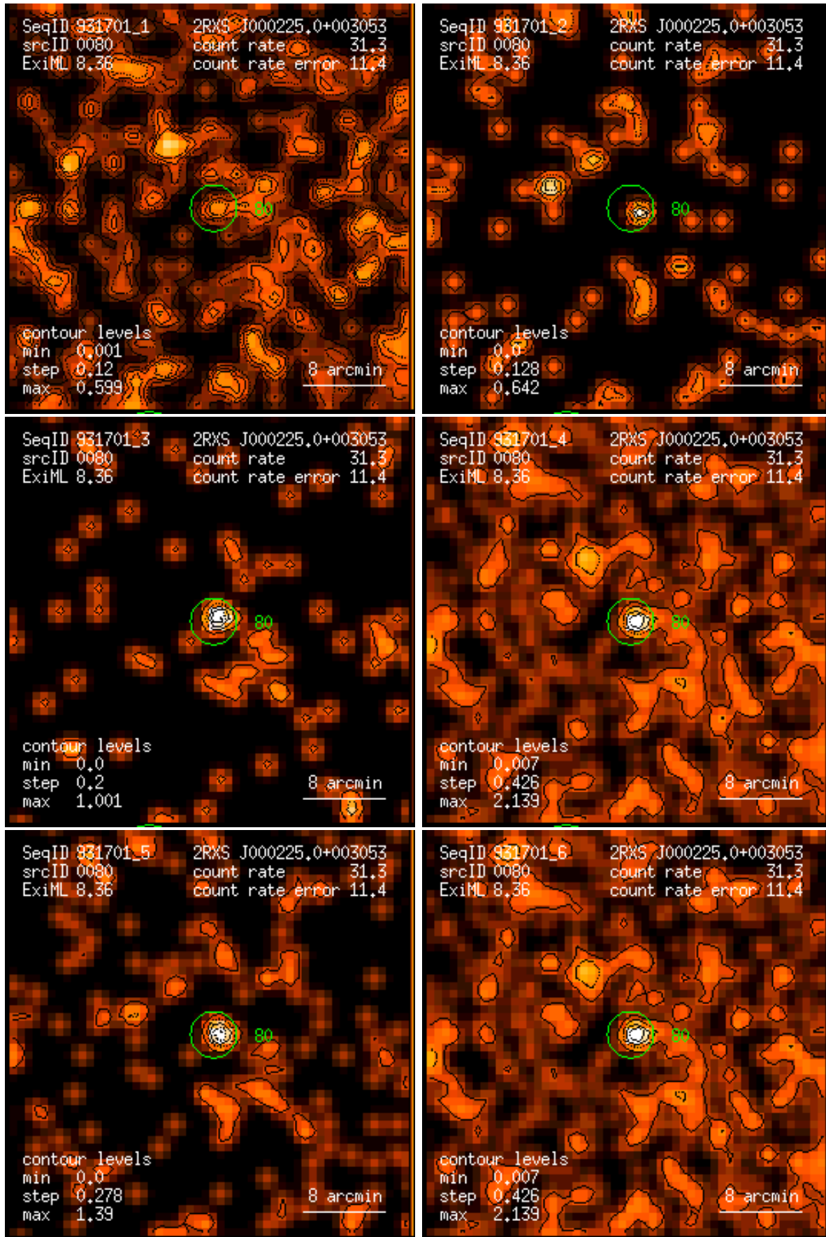
Figure 80: RASS 931701: detection 0080: band rate images, Gaussian filter: (1) PSPC channels 11 – 41, (2) 52 – 90, (3) 91 – 201, (4) 11 – 235, (5) 52 – 201, (6) 11 – 201. Broad band rates in counts/ks. Band rate contour levels in counts/ks/arcmin 2 .
