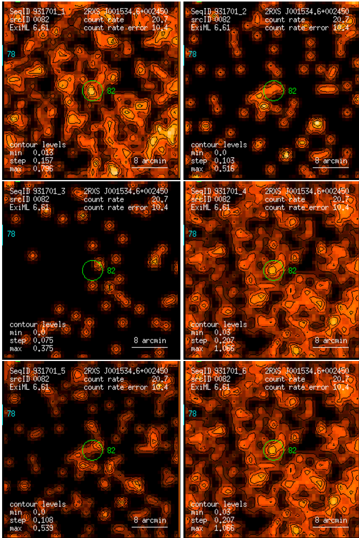
Figure 82: RASS 931701: detection 0082: band rate images, Gaussian filter: (1) PSPC channels 11 – 41, (2) 52 – 90, (3) 91 – 201, (4) 11 – 235, (5) 52 – 201, (6) 11 – 201. Broad band rates in counts/ks. Band rate contour levels in counts/ks/arcmin 2 .
