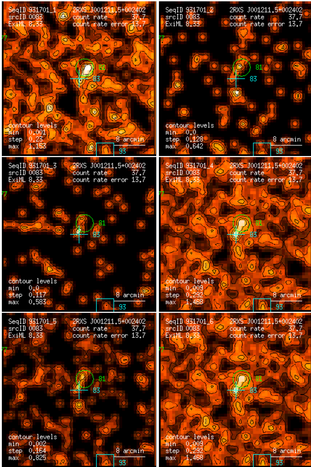
Figure 83: RASS 931701: detection 0083: band rate images, Gaussian filter: (1) PSPC channels 11 – 41, (2) 52 – 90, (3) 91 – 201, (4) 11 – 235, (5) 52 – 201, (6) 11 – 201. Broad band rates in counts/ks. Band rate contour levels in counts/ks/arcmin 2 .
