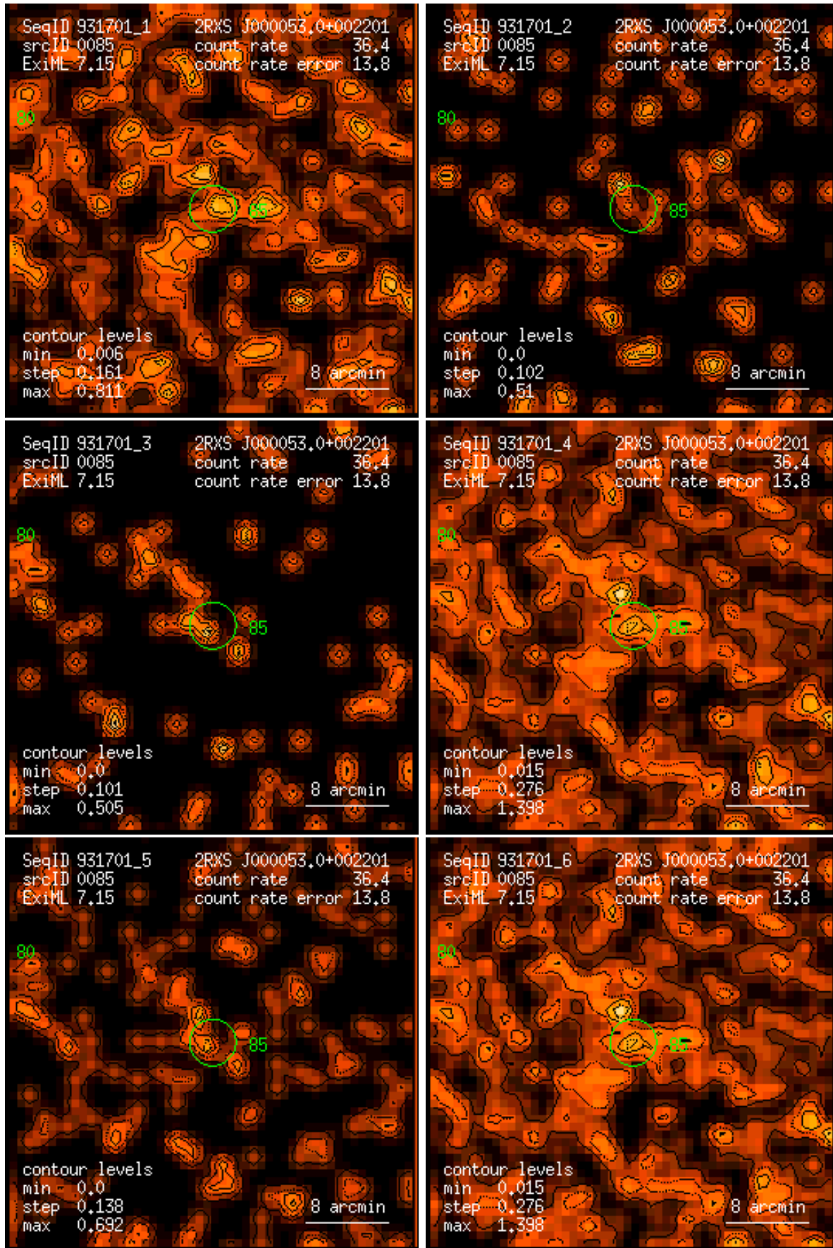
Figure 85: RASS 931701: detection 0085: band rate images, Gaussian filter: (1) PSPC channels 11 – 41, (2) 52 – 90, (3) 91 – 201, (4) 11 – 235, (5) 52 – 201, (6) 11 – 201. Broad band rates in counts/ks. Band rate contour levels in counts/ks/arcmin 2 .
