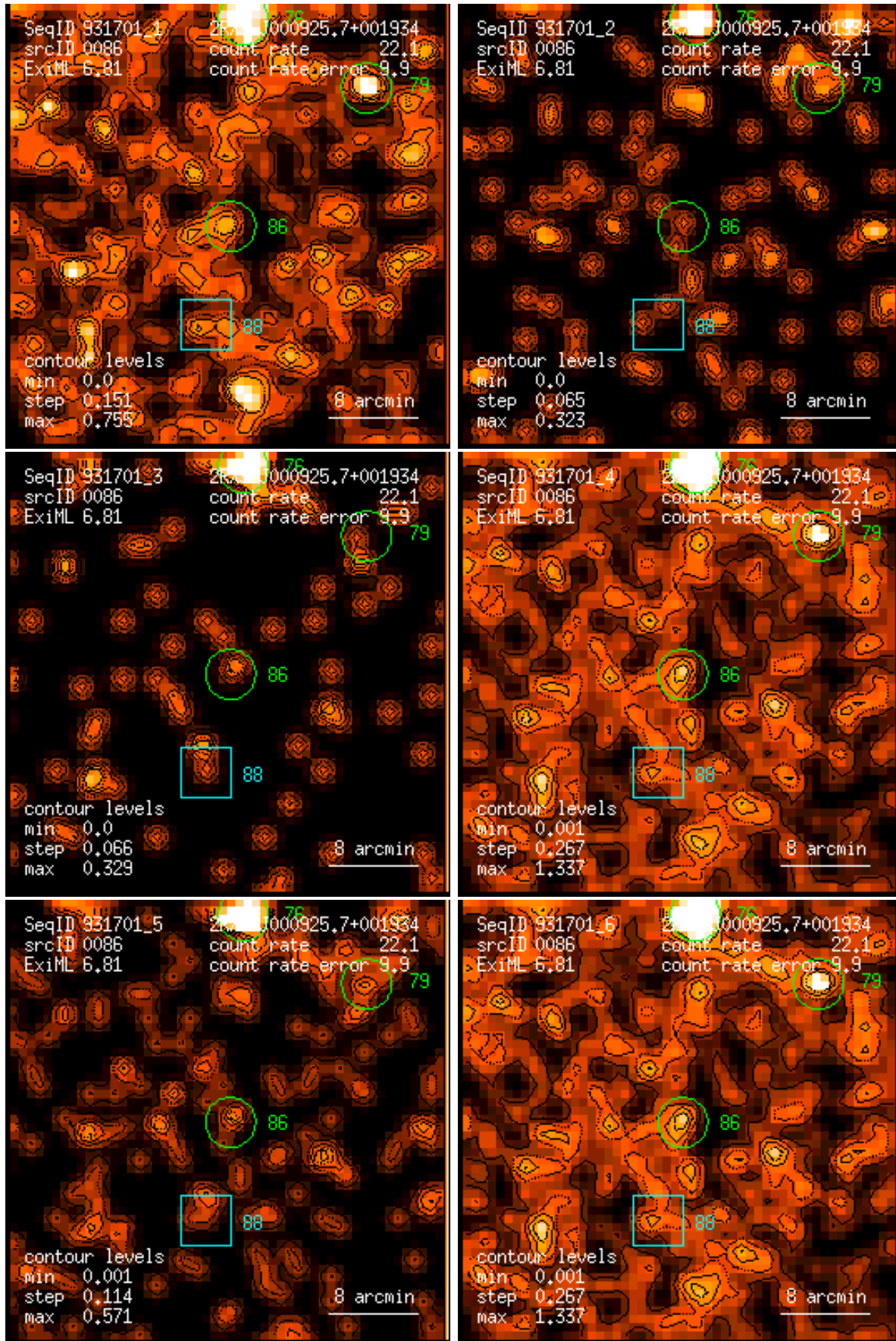
Figure 86: RASS 931701: detection 0086: band rate images, Gaussian filter: (1) PSPC channels 11 – 41, (2) 52 – 90, (3) 91 – 201, (4) 11 – 235, (5) 52 – 201, (6) 11 – 201. Broad band rates in counts/ks. Band rate contour levels in counts/ks/arcmin 2 .
