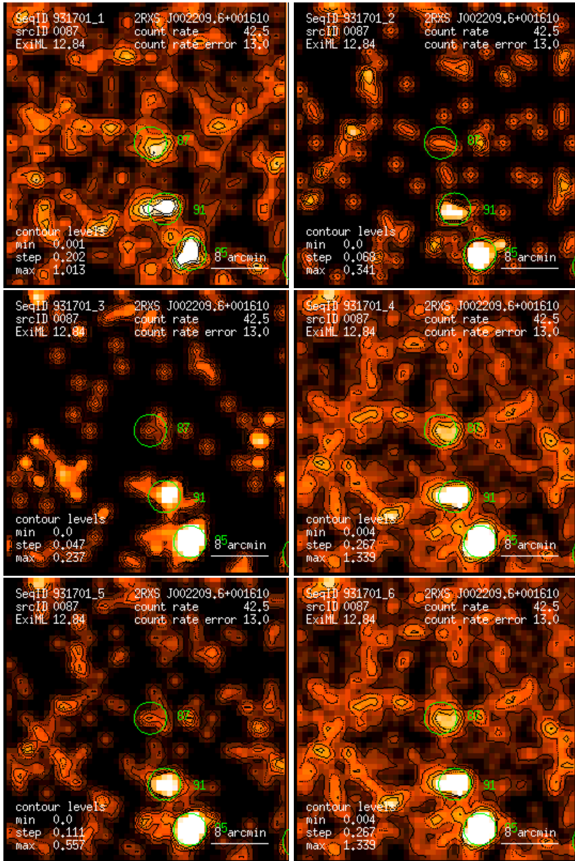
Figure 87: RASS 931701: detection 0087: band rate images, Gaussian filter: (1) PSPC channels 11 – 41, (2) 52 – 90, (3) 91 – 201, (4) 11 – 235, (5) 52 – 201, (6) 11 – 201. Broad band rates in counts/ks. Band rate contour levels in counts/ks/arcmin 2 .
