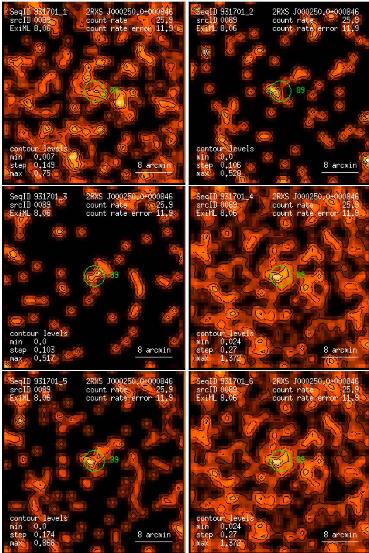
Figure 89: RASS 931701: detection 0089: band rate images, Gaussian filter: (1) PSPC channels 11 – 41, (2) 52 – 90, (3) 91 – 201, (4) 11 – 235, (5) 52 – 201, (6) 11 – 201. Broad band rates in counts/ks. Band rate contour levels in counts/ks/arcmin 2 .
