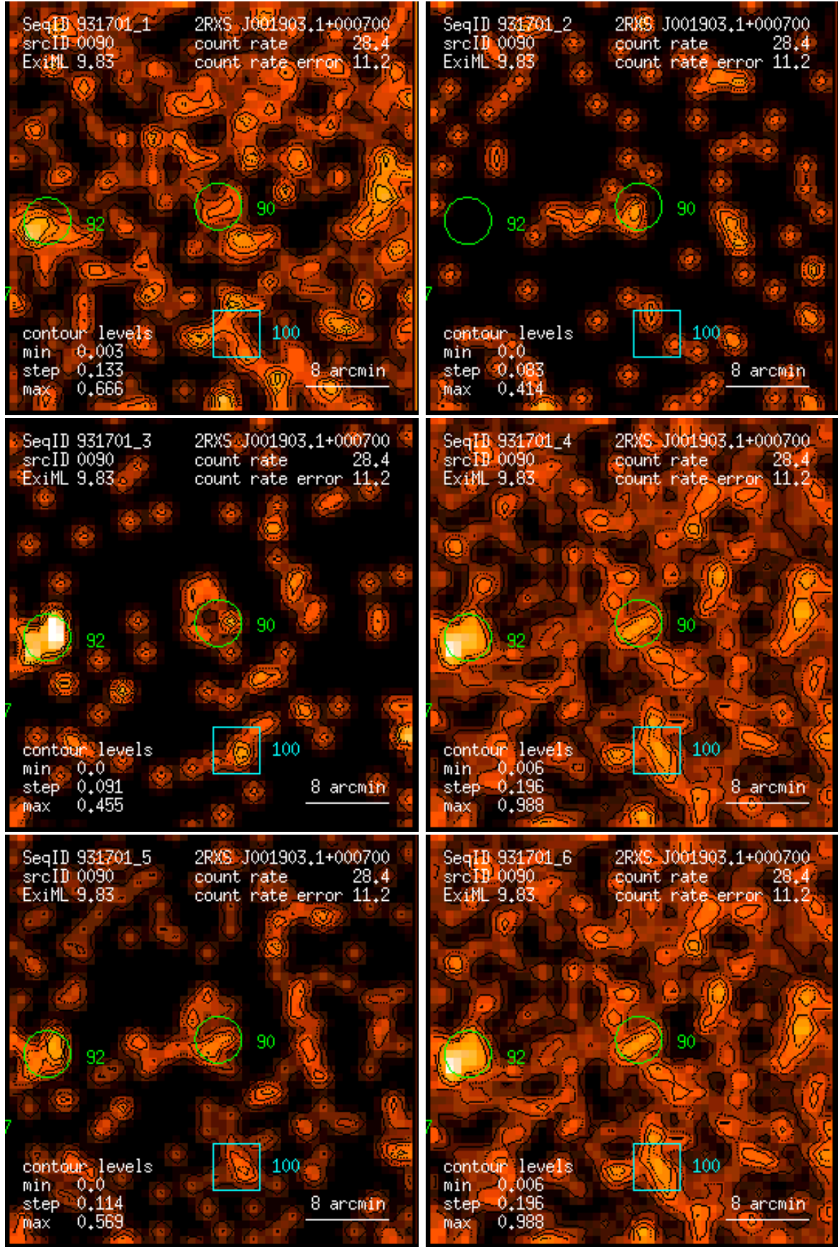
Figure 90: RASS 931701: detection 0090: band rate images, Gaussian filter: (1) PSPC channels 11 – 41, (2) 52 – 90, (3) 91 – 201, (4) 11 – 235, (5) 52 – 201, (6) 11 – 201. Broad band rates in counts/ks. Band rate contour levels in counts/ks/arcmin 2 .
