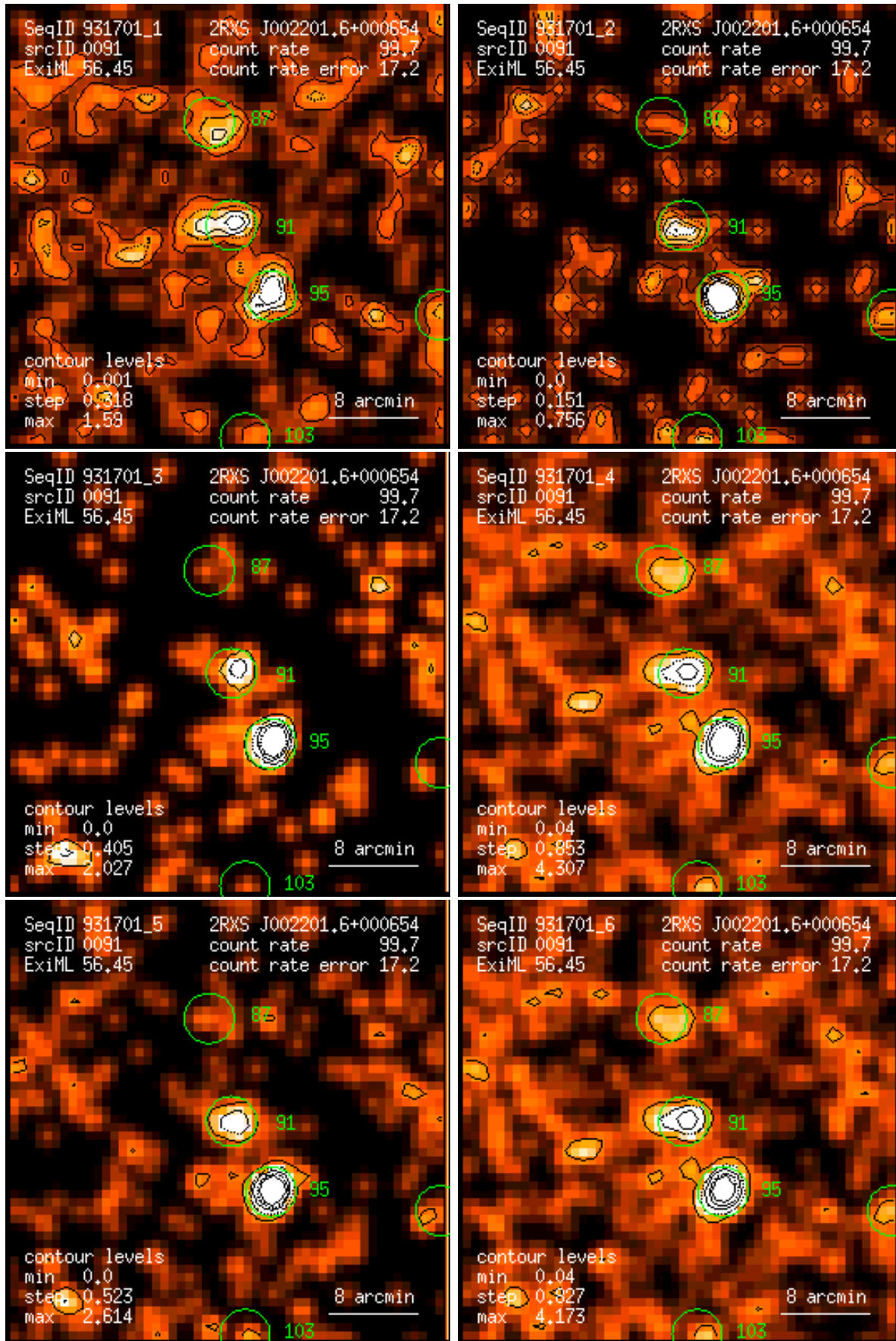
Figure 91: RASS 931701: detection 0091: band rate images, Gaussian filter: (1) PSPC channels 11 – 41, (2) 52 – 90, (3) 91 – 201, (4) 11 – 235, (5) 52 – 201, (6) 11 – 201. Broad band rates in counts/ks. Band rate contour levels in counts/ks/arcmin 2 .
