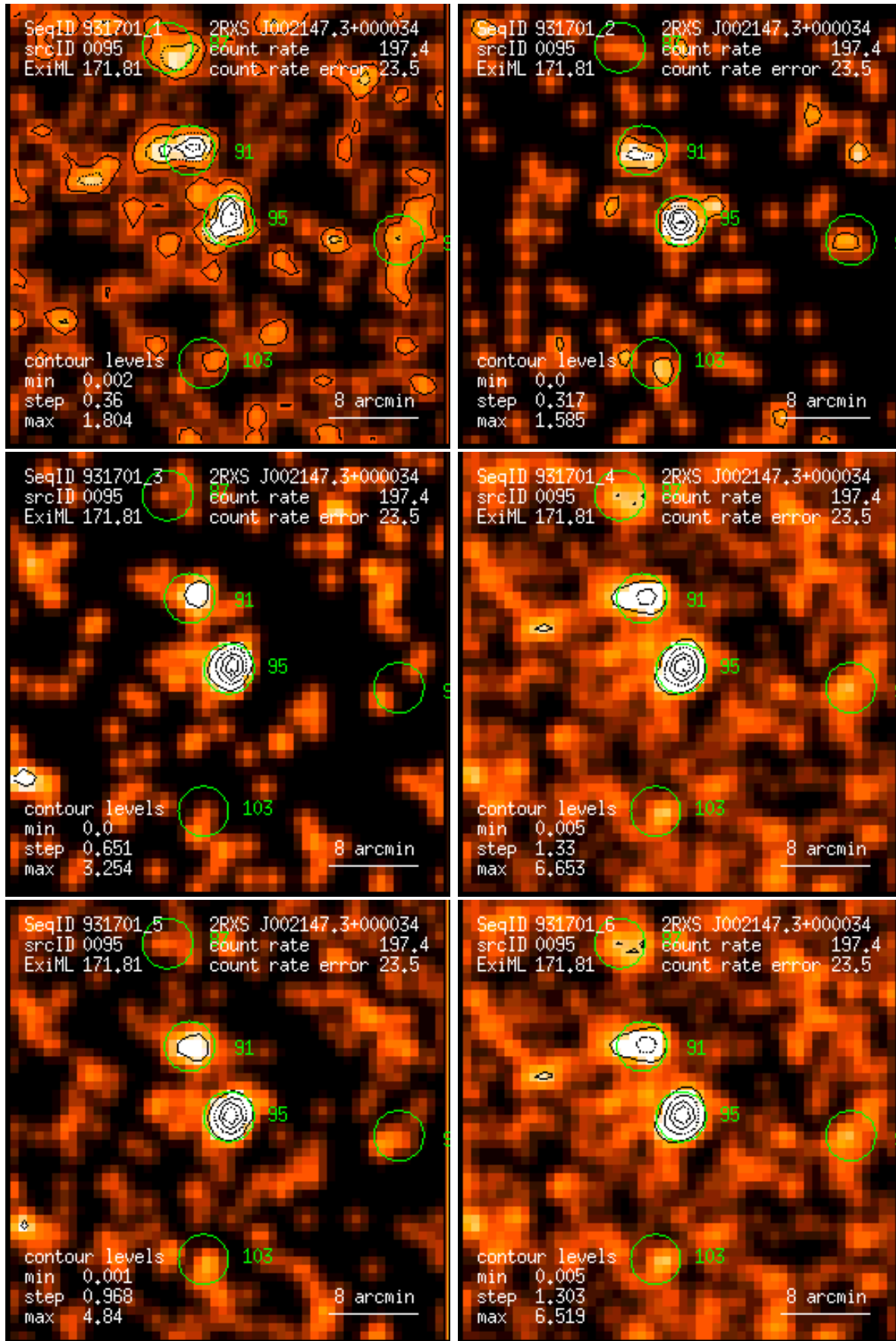
Figure 95: RASS 931701: detection 0095: band rate images, Gaussian filter: (1) PSPC channels 11 – 41, (2) 52 – 90, (3) 91 – 201, (4) 11 – 235, (5) 52 – 201, (6) 11 – 201. Broad band rates in counts/ks. Band rate contour levels in counts/ks/arcmin 2 .
