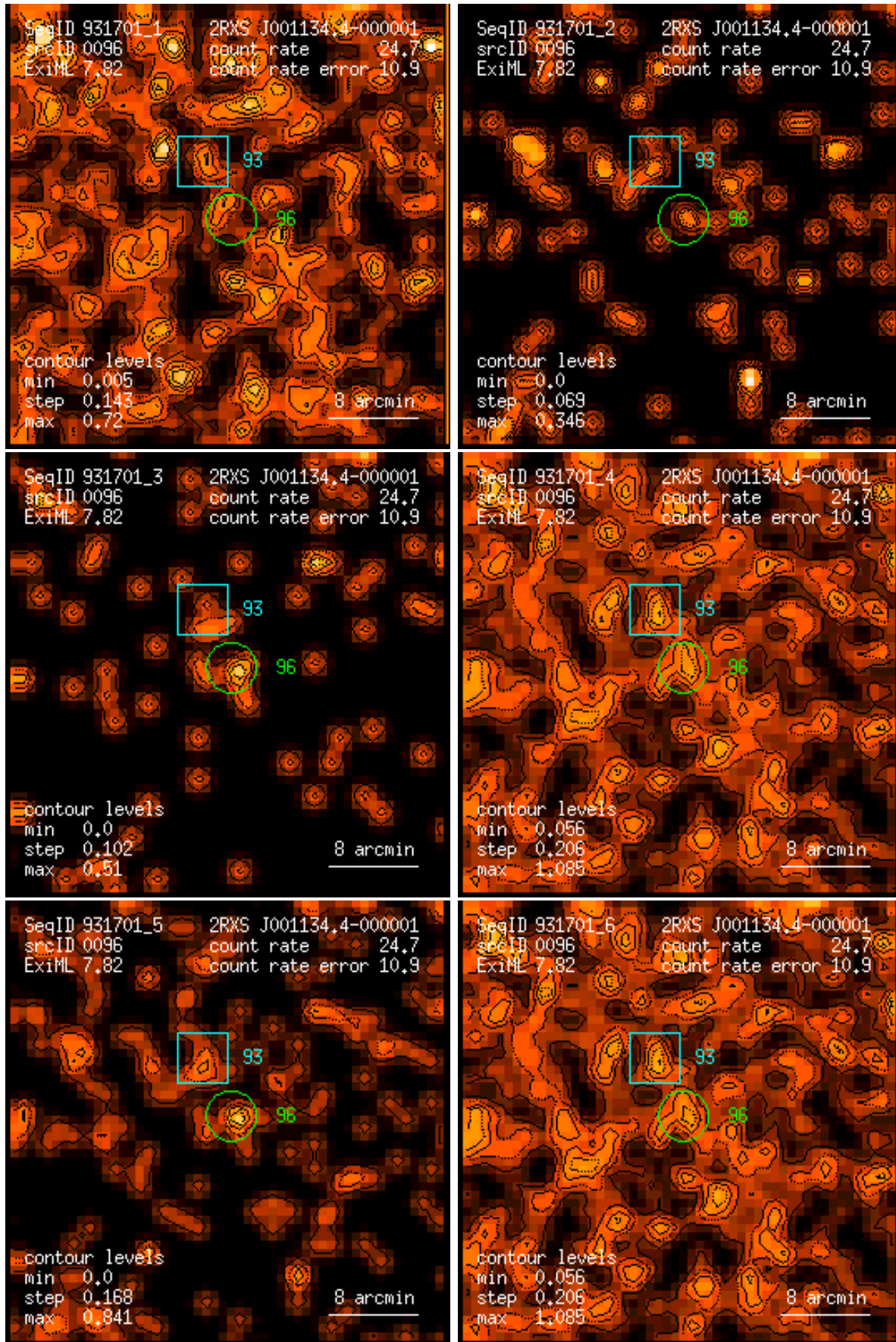
Figure 96: RASS 931701: detection 0096: band rate images, Gaussian filter: (1) PSPC channels 11 – 41, (2) 52 – 90, (3) 91 – 201, (4) 11 – 235, (5) 52 – 201, (6) 11 – 201. Broad band rates in counts/ks. Band rate contour levels in counts/ks/arcmin 2 .
