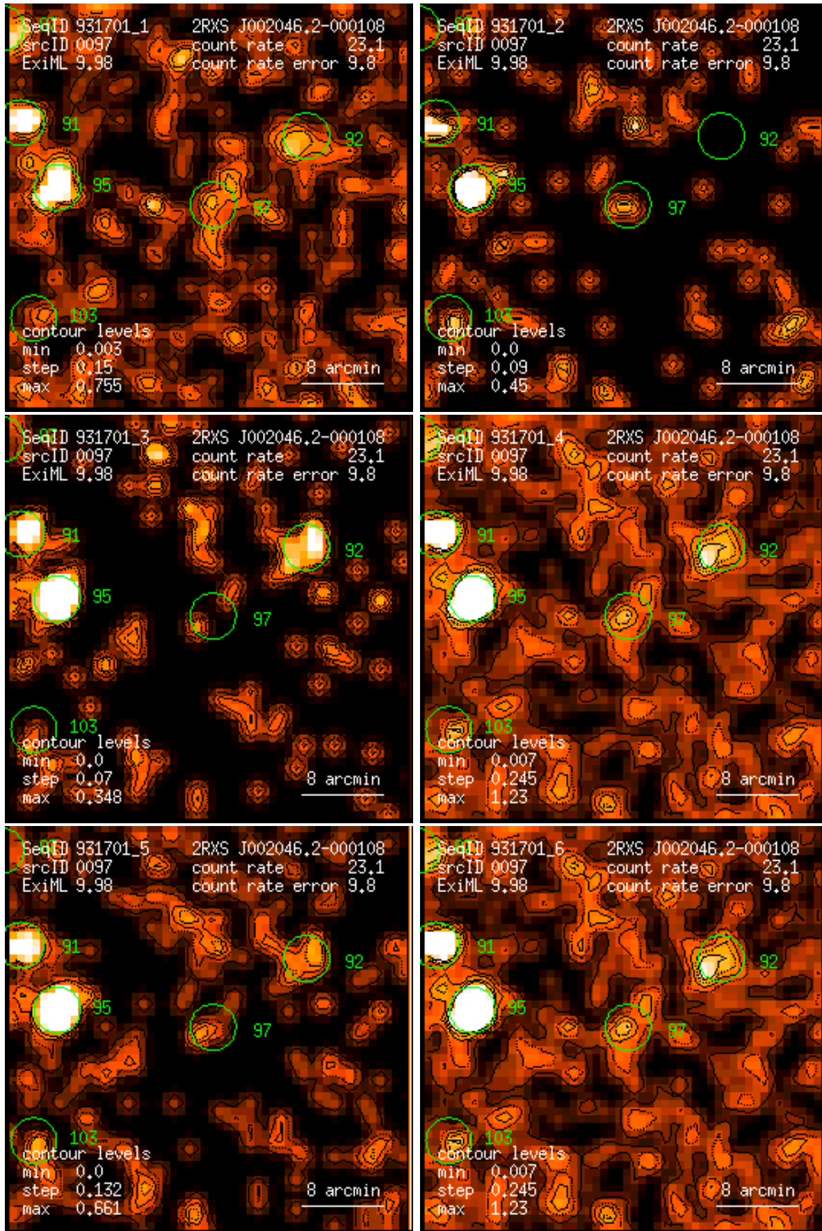
Figure 97: RASS 931701: detection 0097: band rate images, Gaussian filter: (1) PSPC channels 11 – 41, (2) 52 – 90, (3) 91 – 201, (4) 11 – 235, (5) 52 – 201, (6) 11 – 201. Broad band rates in counts/ks. Band rate contour levels in counts/ks/arcmin 2 .
