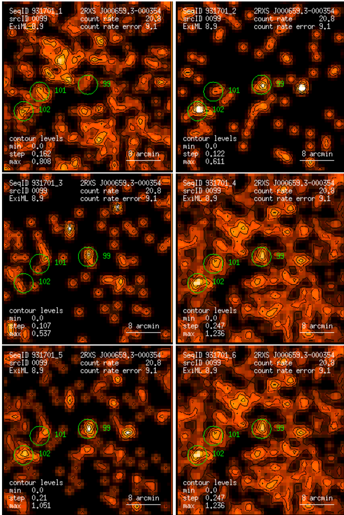
Figure 99: RASS 931701: detection 0099: band rate images, Gaussian filter: (1) PSPC channels 11 – 41, (2) 52 – 90, (3) 91 – 201, (4) 11 – 235, (5) 52 – 201, (6) 11 – 201. Broad band rates in counts/ks. Band rate contour levels in counts/ks/arcmin 2 .
