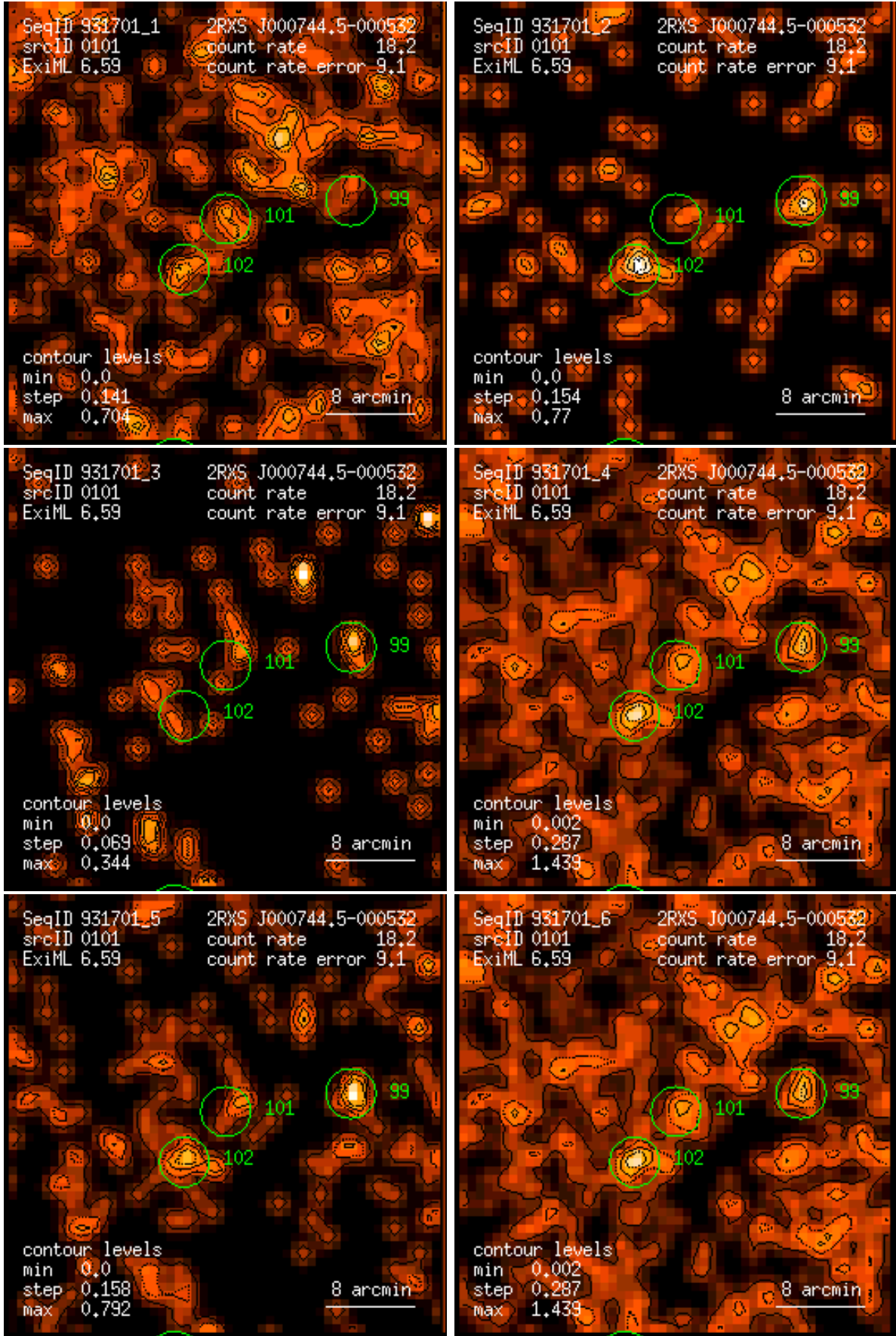
Figure 101: RASS 931701: detection 0101: band rate images, Gaussian filter: (1) PSPC channels 11 – 41, (2) 52 – 90, (3) 91 – 201, (4) 11 – 235, (5) 52 – 201, (6) 11 – 201. Broad band rates in counts/ks. Band rate contour levels in counts/ks/arcmin 2 .
