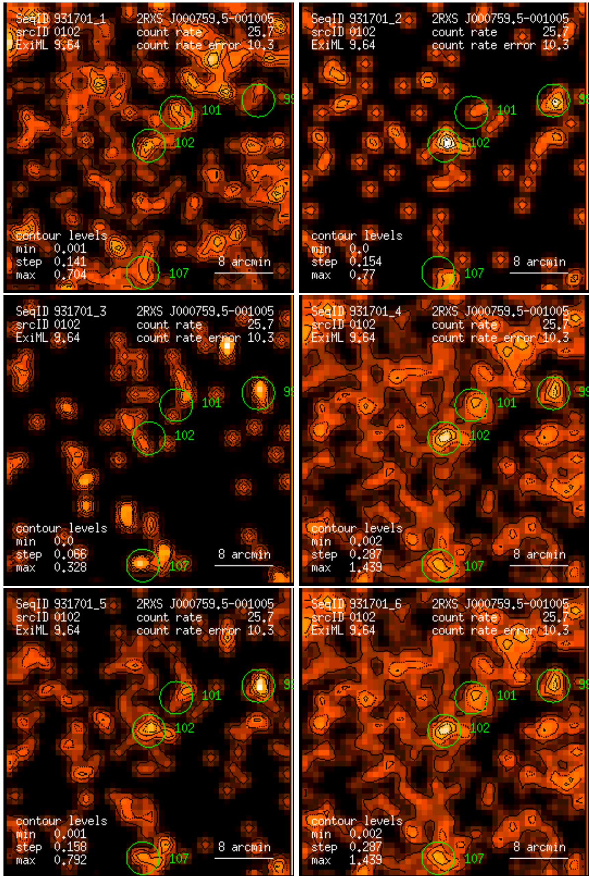
Figure 102: RASS 931701: detection 0102: band rate images, Gaussian filter: (1) PSPC channels 11 – 41, (2) 52 – 90, (3) 91 – 201, (4) 11 – 235, (5) 52 – 201, (6) 11 – 201. Broad band rates in counts/ks. Band rate contour levels in counts/ks/arcmin 2 .
