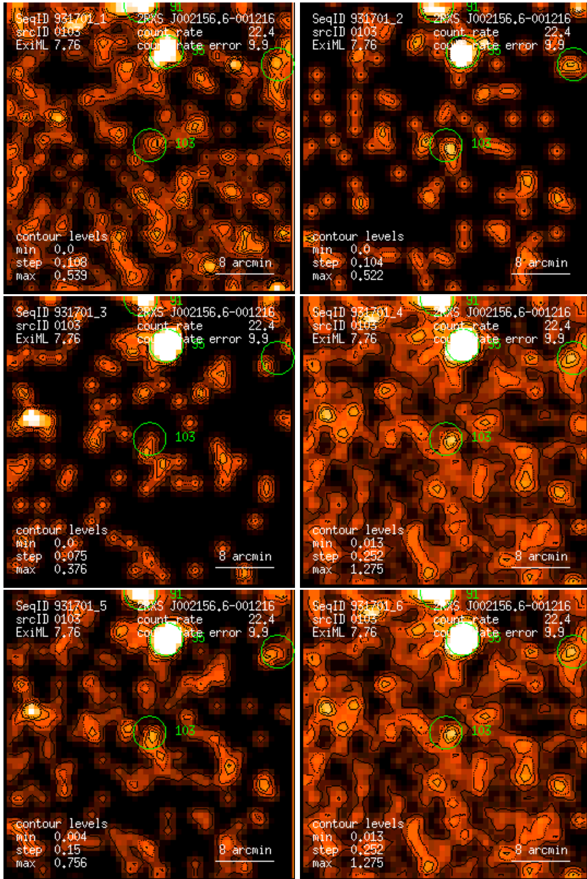
Figure 103: RASS 931701: detection 0103: band rate images, Gaussian filter: (1) PSPC channels 11 – 41, (2) 52 – 90, (3) 91 – 201, (4) 11 – 235, (5) 52 – 201, (6) 11 – 201. Broad band rates in counts/ks. Band rate contour levels in counts/ks/arcmin 2 .
