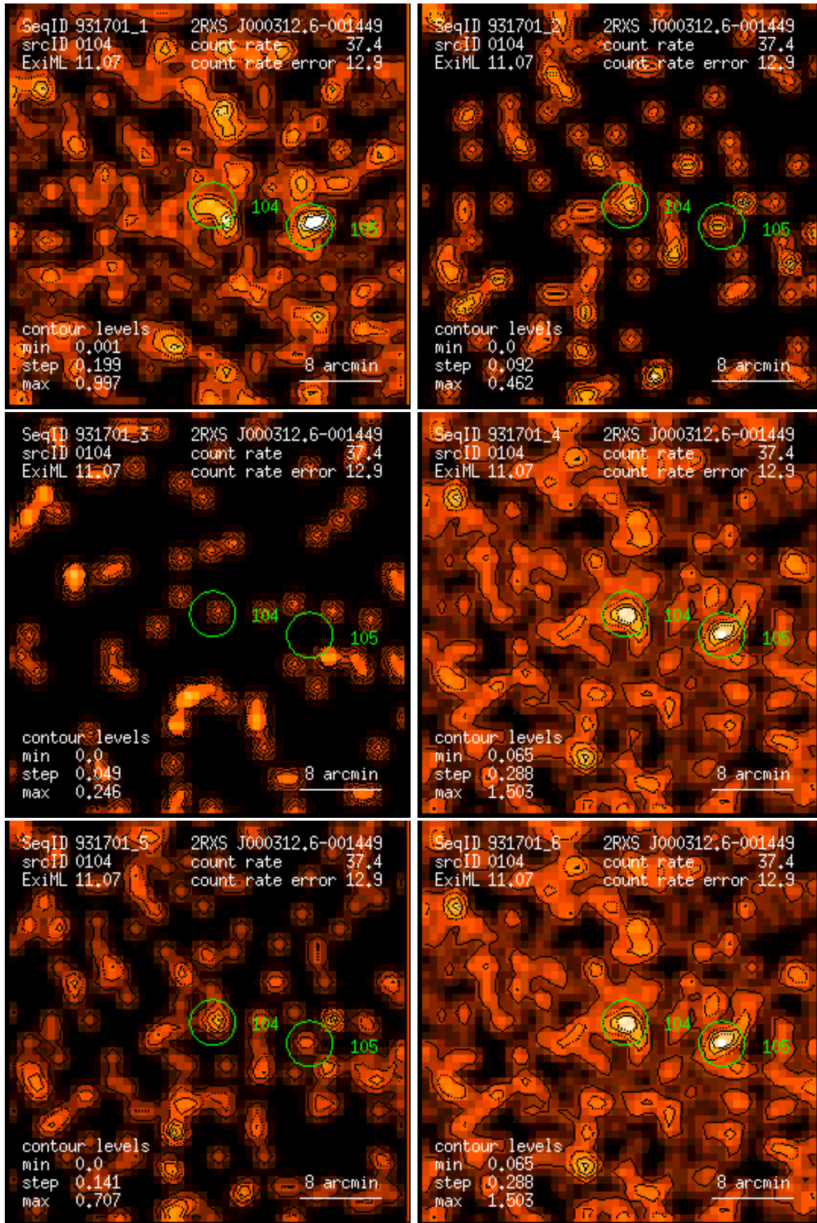
Figure 104: RASS 931701: detection 0104: band rate images, Gaussian filter: (1) PSPC channels 11 – 41, (2) 52 – 90, (3) 91 – 201, (4) 11 – 235, (5) 52 – 201, (6) 11 – 201. Broad band rates in counts/ks. Band rate contour levels in counts/ks/arcmin 2 .
