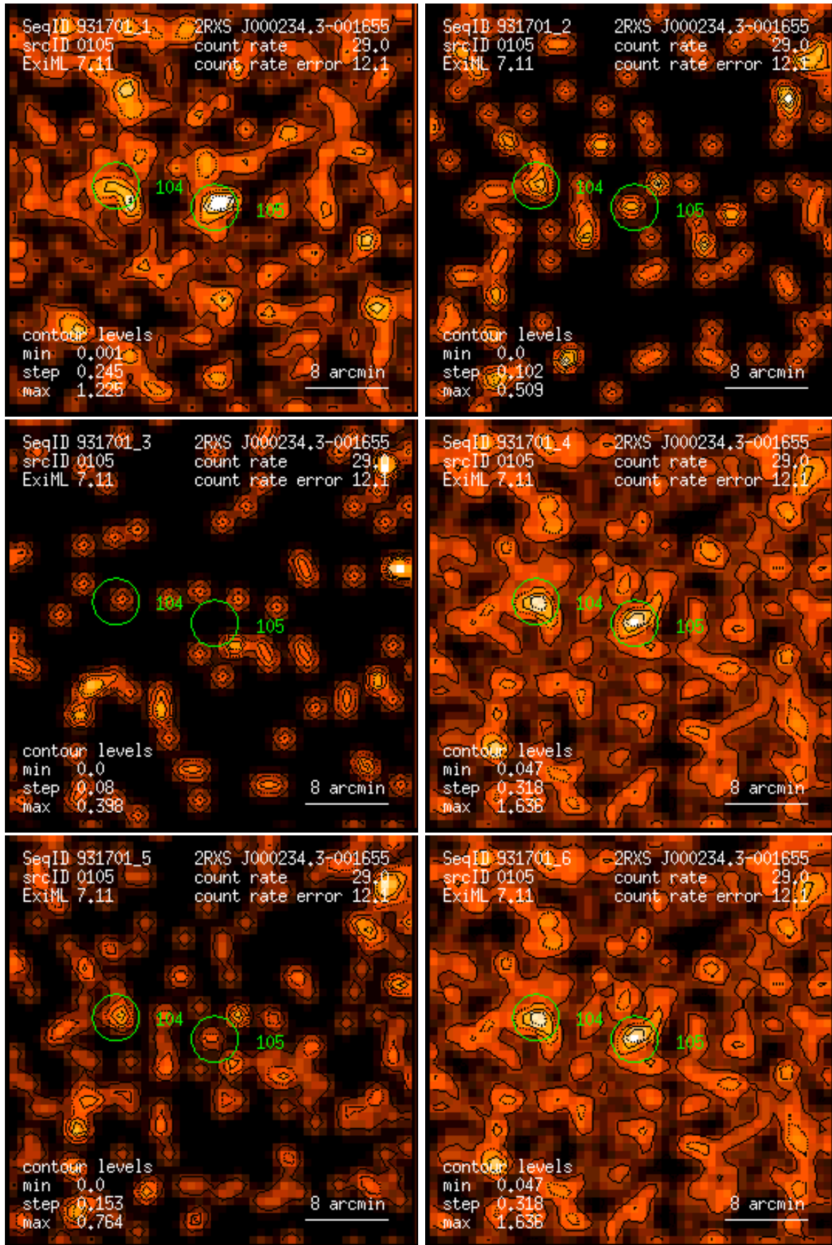
Figure 105: RASS 931701: detection 0105: band rate images, Gaussian filter: (1) PSPC channels 11 – 41, (2) 52 – 90, (3) 91 – 201, (4) 11 – 235, (5) 52 – 201, (6) 11 – 201. Broad band rates in counts/ks. Band rate contour levels in counts/ks/arcmin 2 .
