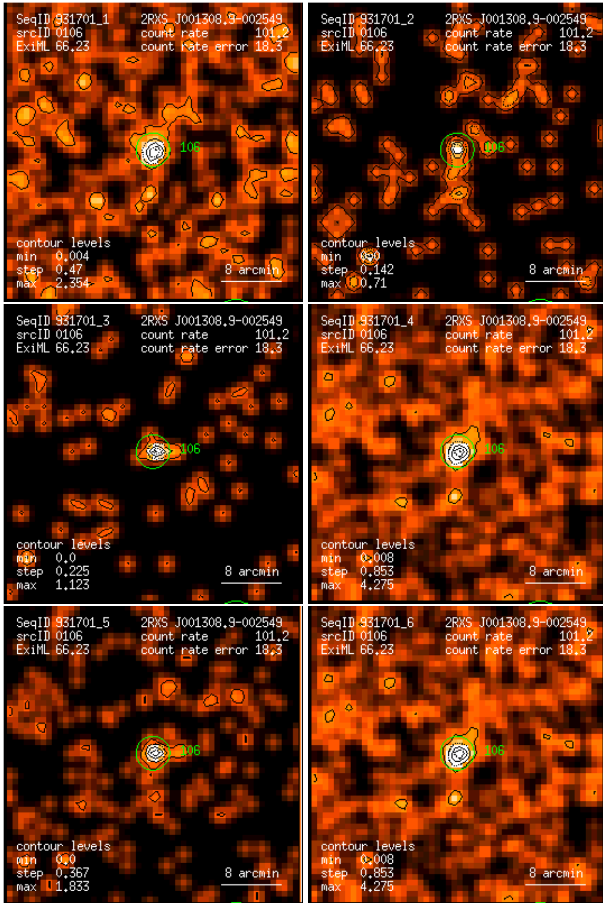
Figure 106: RASS 931701: detection 0106: band rate images, Gaussian filter: (1) PSPC channels 11 – 41, (2) 52 – 90, (3) 91 – 201, (4) 11 – 235, (5) 52 – 201, (6) 11 – 201. Broad band rates in counts/ks. Band rate contour levels in counts/ks/arcmin 2 .
