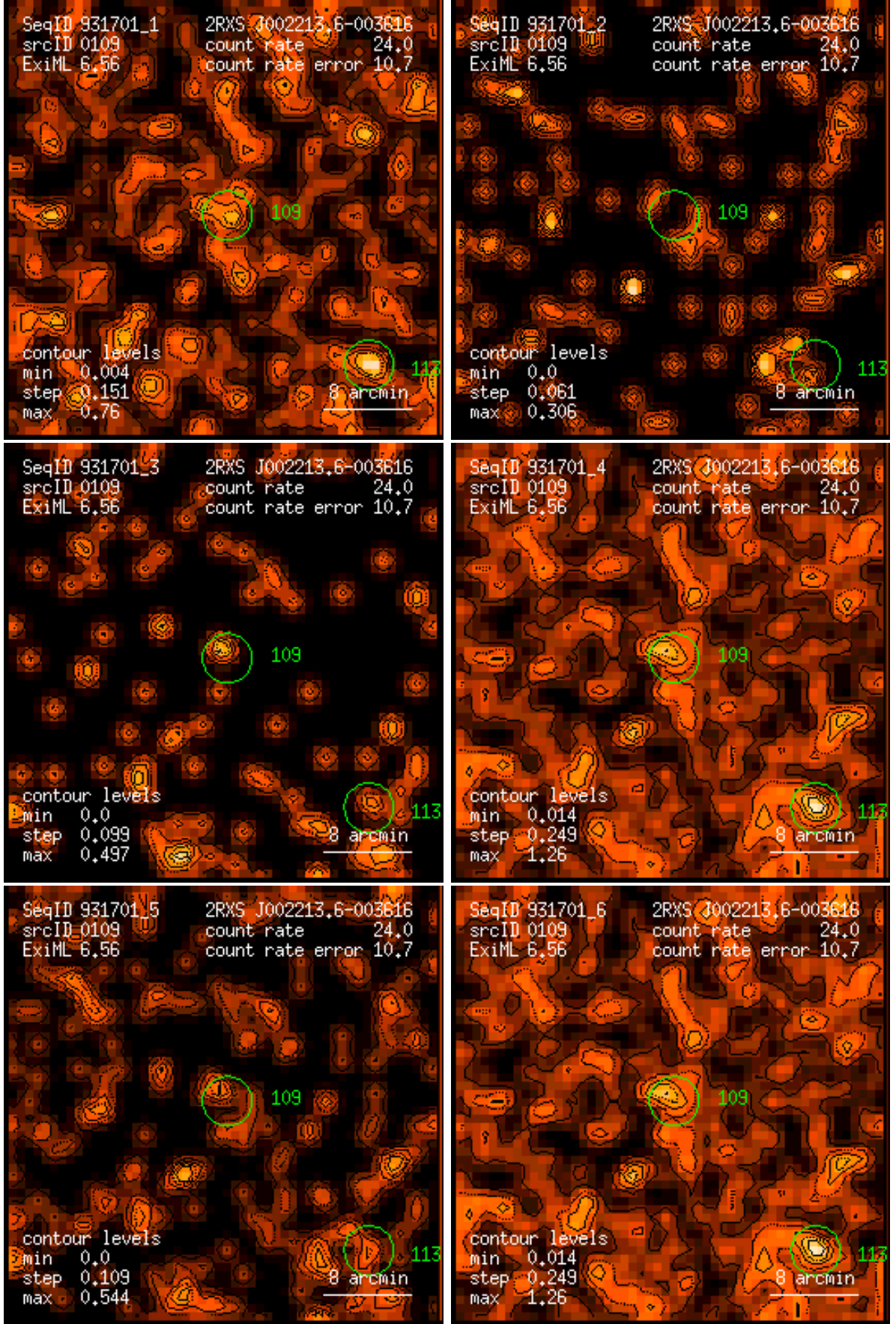
Figure 109: RASS 931701: detection 0109: band rate images, Gaussian filter: (1) PSPC channels 11 – 41, (2) 52 – 90, (3) 91 – 201, (4) 11 – 235, (5) 52 – 201, (6) 11 – 201. Broad band rates in counts/ks. Band rate contour levels in counts/ks/arcmin 2 .
