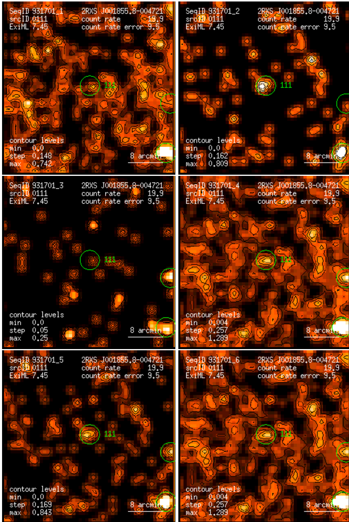
Figure 111: RASS 931701: detection 0111: band rate images, Gaussian filter: (1) PSPC channels 11 – 41, (2) 52 – 90, (3) 91 – 201, (4) 11 – 235, (5) 52 – 201, (6) 11 – 201. Broad band rates in counts/ks. Band rate contour levels in counts/ks/arcmin 2 .
