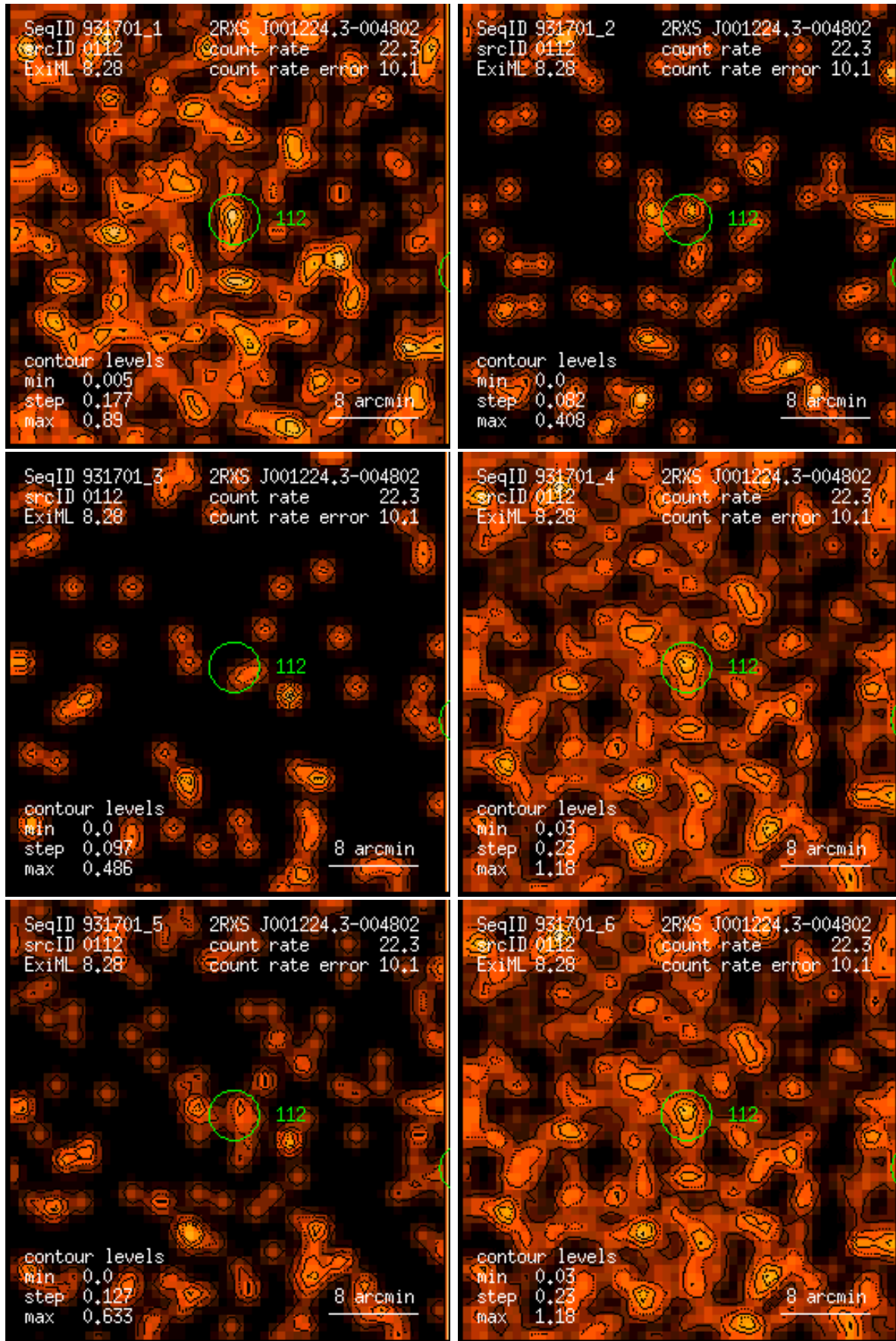
Figure 112: RASS 931701: detection 0112: band rate images, Gaussian filter: (1) PSPC channels 11 – 41, (2) 52 – 90, (3) 91 – 201, (4) 11 – 235, (5) 52 – 201, (6) 11 – 201. Broad band rates in counts/ks. Band rate contour levels in counts/ks/arcmin 2 .
