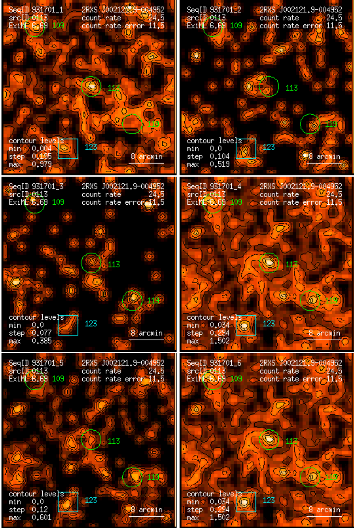
Figure 113: RASS 931701: detection 0113: band rate images, Gaussian filter: (1) PSPC channels 11 – 41, (2) 52 – 90, (3) 91 – 201, (4) 11 – 235, (5) 52 – 201, (6) 11 – 201. Broad band rates in counts/ks. Band rate contour levels in counts/ks/arcmin 2 .
