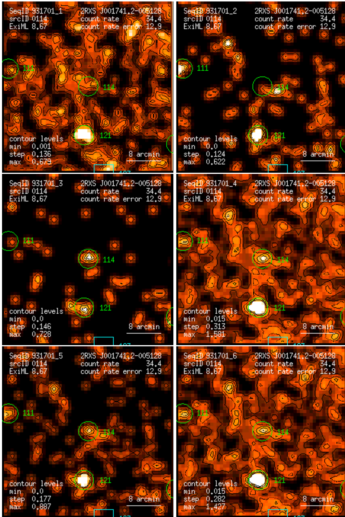
Figure 114: RASS 931701: detection 0114: band rate images, Gaussian filter: (1) PSPC channels 11 – 41, (2) 52 – 90, (3) 91 – 201, (4) 11 – 235, (5) 52 – 201, (6) 11 – 201. Broad band rates in counts/ks. Band rate contour levels in counts/ks/arcmin 2 .
